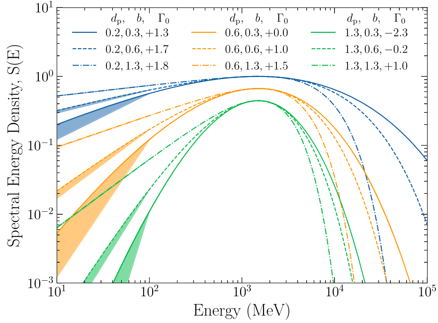
Figure 15. Realizations of the PLEC4 model for three values of the peak curvature, d_p = 0.2, 0.6 , and 1.3 , and the asymmetry parameter b = 0.3, 0.6 , and 1.3 . We set E_p = E_0 = 1 GeV, which uniquely determines \Gamma and \Gamma_0 . The SEDs are normalized to 1 at E_p but offset by 50% for clarity. Each curve is labeled with the tuple (d, b, \Gamma_0) . The shaded regions show the difference between the SED and the asymptotic power law, normalized to 0.1 GeV.
