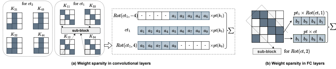
Figure 4. (a) The weight sparse pattern in convolutional layers. For the same ct , their weight sparse patterns must be the same. For different ct , the weight sparse pattern may change. (b) The weight sparse pattern in FC layers is in a diagonal-wise shape.
