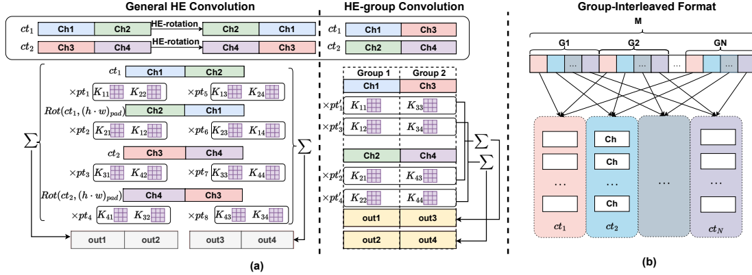
Figure 3. (a) an example of HE convolution which generates 4 output channels from the 4 input channels with 3 \times 3 kernels. By HE-group convolution, we only need 2 group-interleaved encoded cts to multiply with corresponding pts and sum up to get the output channels data. (b) proposed HE-group convolution by a group-interleaved format.
