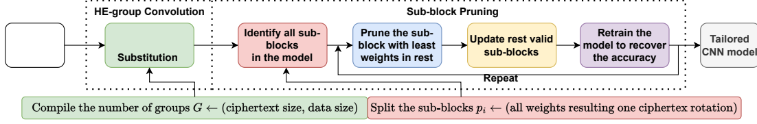
Figure 2. An overview of SpENCNN for optimizing HE-based CNN inference, mainly consists of two orthogonal techniques to generate a tailored model: (1) HE-group Convolution (outer-rotation optimization), and (2) Sub-block Pruning (inner-rotation optimization).
