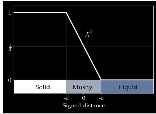
Fig. 3. Illustration of the relaxed phase function \chi^\varepsilon(\rho) = \frac{(1-\rho/\varepsilon)^+}{2} \wedge 1 .
