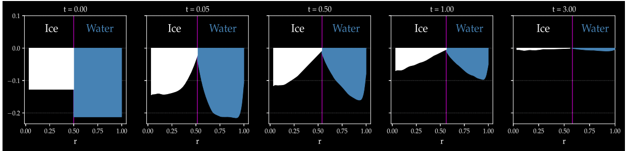
Fig. 10. Two-phase, supercooled Stefan problem without surface tension ( d = 2 ) discussed in Section 4.1.2. Temperature (vertical axis) in the liquid ( u^1 ) and the solid ( u^2 ) retrieved using Monte Carlo simulation and kernel density estimation (KDE). At t = 3 , both phases are already close to their equilibrium temperature u_\infty^1 = u_\infty^2 = 0 and long term radius r_\infty \approx 0.59 .
