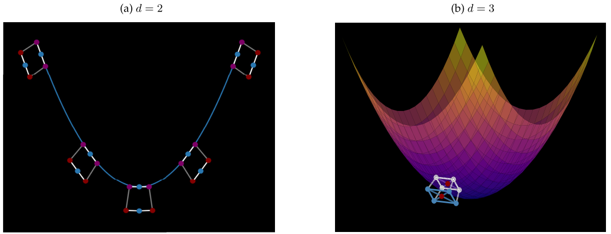
Fig. 4. Dilation technique to capture the mean curvature of codimension 1 interfaces in \mathbb{R}^d , d = 2, 3 .
