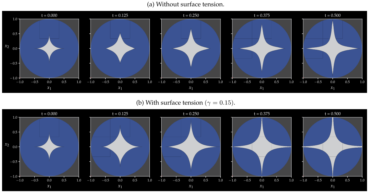
Fig. 16. Two-phase Stefan problem with diamond-shaped initial solid region ( d = 2 ) and supercooled liquid. Evolution of the solid region over time.
