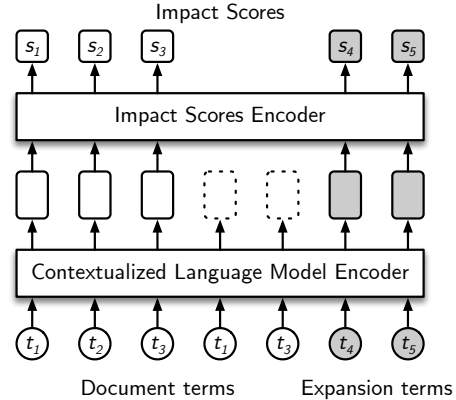
Figure 1: Neural network architecture of DeepImpact.
