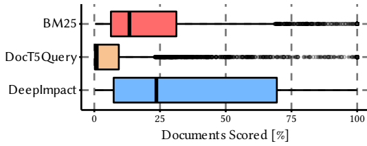
Figure 2: Relative percentage of documents scored (as compared to an exhaustive algorithm) with MaxScore for k = 1000 over the MSMARCO Dev Queries.
