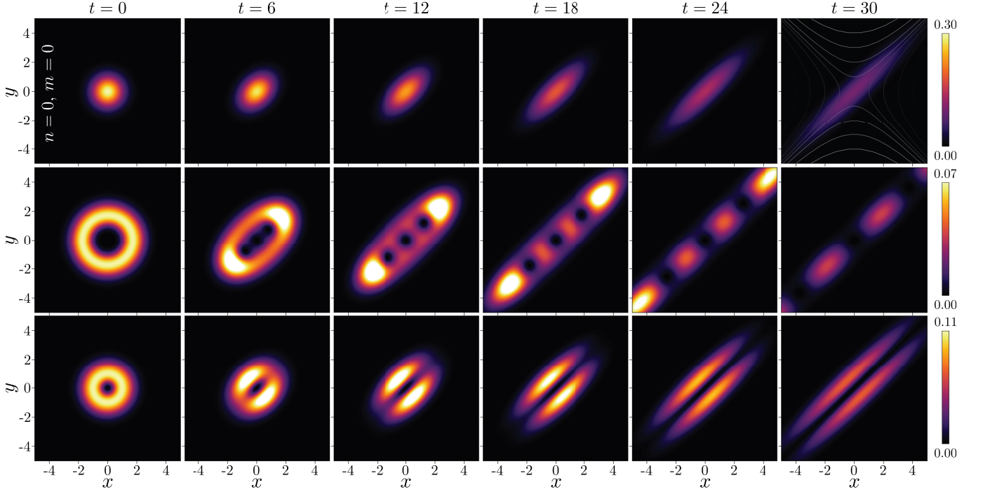
FIG. 3. Density |\langle x, y | n, m \rangle_t|^2 of the time evolved Fock states. After a small transient evolution, which is longer for higher cyclotron index n , the dynamics is well captured by isopotential flow of guiding centers. As a guide to the eye allowing to visualize the guiding center drift, some isopotential lines of the rotating saddle potential \varepsilon(x^2 - y^2) are shown on the topmost right panel with solid lines using a gray scale, which goes from black (negative) to white (positive) values.
