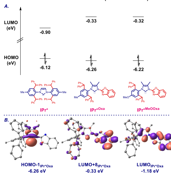
Fig. 6. (A) HOMO and LUMO energy levels (eV). (B) HOMO-1, LUMO+8 and LUMO (eV) of \text{IPr}^*\text{Oxa} calculated at B3LYP 6-311++g(d,p). See SI.
