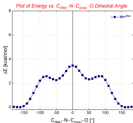
Fig. 7. Rotational profile of IPr*Oxa ( \Delta E , kcal/mol, vs. C(\text{Me})-N-C(\text{oxa})-O [ ^\circ ]).
