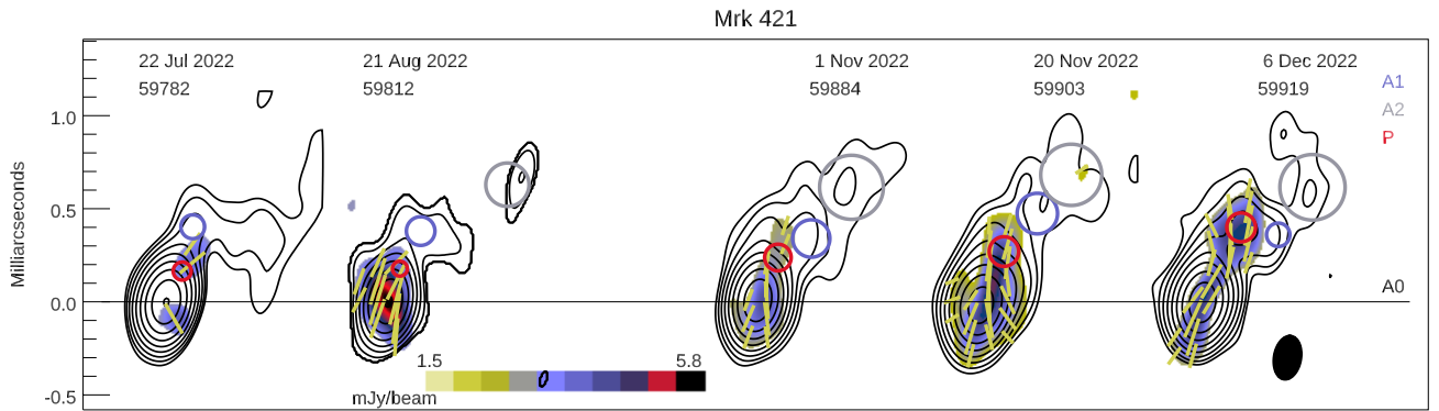
Fig. 7. VLBA total (contours) and polarized (color scale) intensity images of Mrk 421 at 43 GHz. The peak of the total intensity is 295 mJy beam ^{-1} . Yellow linear segments within the images indicate the direction of polarization, the black horizontal line marks the position of the core, A0, and colored circles indicate locations of jet features A1 (blue), A2 (gray), and P (red). Images are convolved with the same elliptical Gaussian beam, which is shown in the bottom-right corner by a black ellipse.
