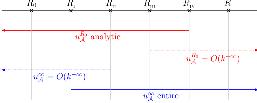
FIG. 1.1. The regions where u_{\mathcal{A}}^{R_0} and u_{\mathcal{A}}^{\infty} appearing in Theorem B are analytic, entire, or O(k^{-\infty}) .
