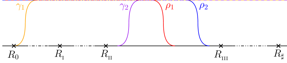
FIG. 3.2. The cut-off functions \rho_1, \rho_2, \gamma_1, \gamma_2 . \rho_1 is used in §3.3.2, \rho_2 in §3.3.3, and \gamma_1 and \gamma_2 in §3.3.4.
