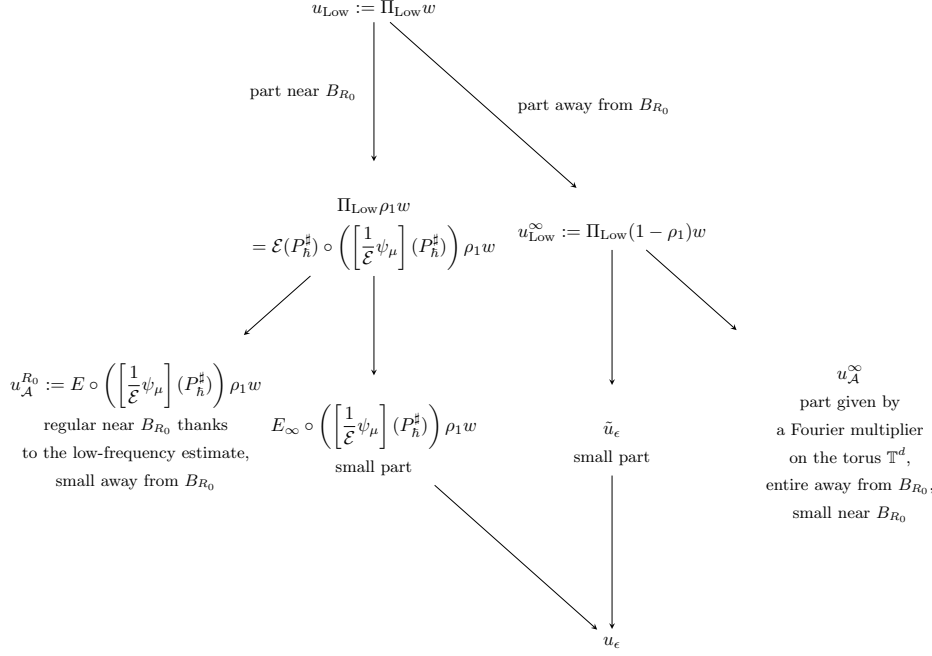
FIG. 3.3. The splitting of u_{\text{Low}}
