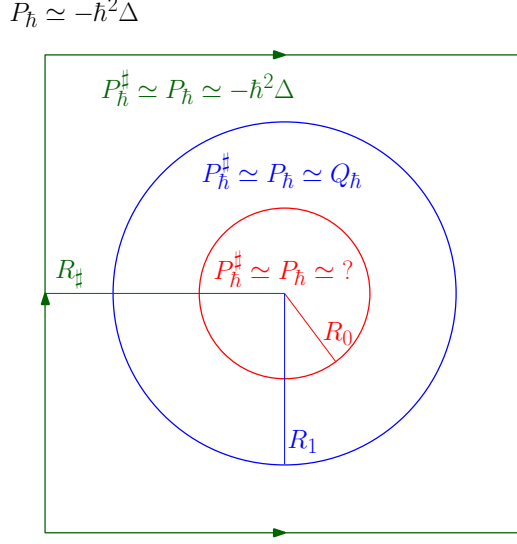
FIG. 2.1. The black-box setting. The symbol \simeq is used to denote equality in the sense of (BB2) and (2.5).
