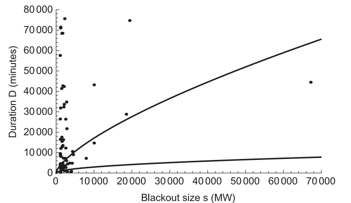
Fig. 7. Dots show improved NERC data for blackout duration versus size for larger blackouts. Upper curve D = 29.5s^{0.69} fits a power law to the sublinear, large blackout data. Since lower curve D = 29.5s^{0.5} lies well below most of data, it is a conservative lower bound.
