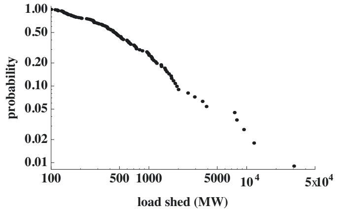
Fig. 6. CCDF of load shed in WECC blackouts.
