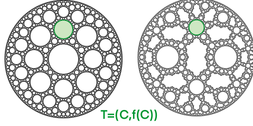
FIGURE 2. The left-hand side is the limit set of a convex-cocompact Kleinian group \Gamma and the right-hand side is the limit set of a quasi-conformal deformation, say, \rho_0 , of \Gamma .
