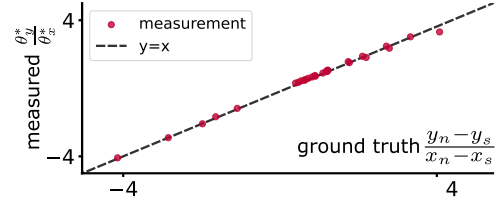
(b) impact source direction: recovered vs. ground truth
