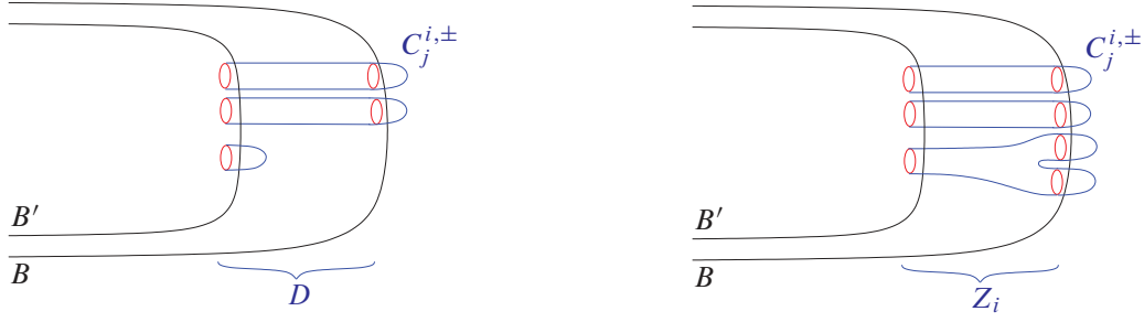
Figure 2. A schematic picture of the fillings E_w (left) and E'_w (right). For simplicity, we drew the components of the cable side by side, rather than nested.
