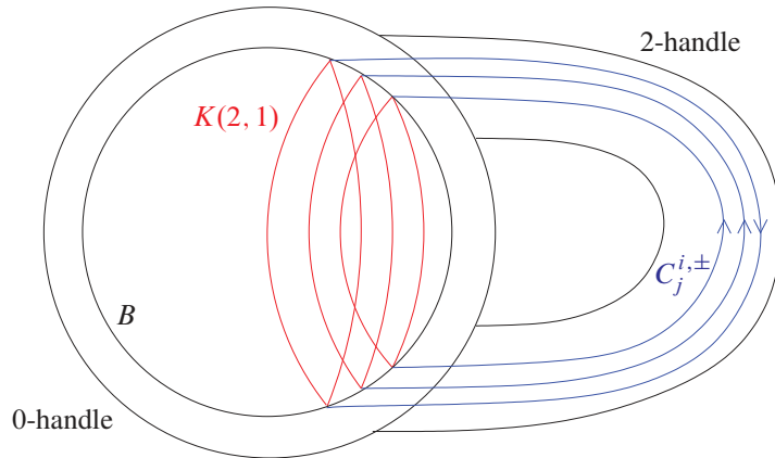
Figure 1. A generator for \mathcal{S}_0^N(W; \emptyset, 0) .
