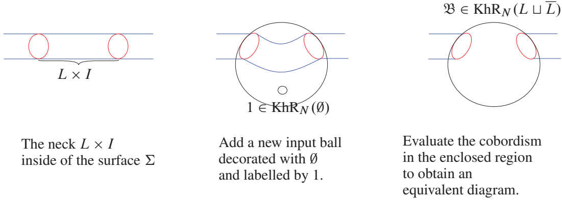
Figure 4. Proof of the neck-cutting lemma.
