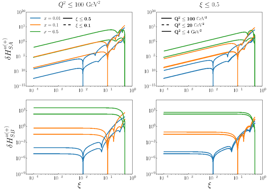
FIG. 5. Top row: results for \delta H_5 from Eq. (22) for type A SGPDs as a function of \xi , for three values of x \gtrsim 0.01; 0.1; 0.5 . Bottom row: Results for \delta H_5 from Eq. (22) for type B SGPDs as a function of \xi , for three values of x \gtrsim 0.01; 0.1; 0.5 . In both cases, the left panels indicate results for cuts in the simulated CFF data in \xi , and the results in the right panels illustrate constraints on the SGPDs associated with cuts in Q^2 on the simulated CFF data. In each row the solid lines are the same and represent constraints from the full simulated dataset.
