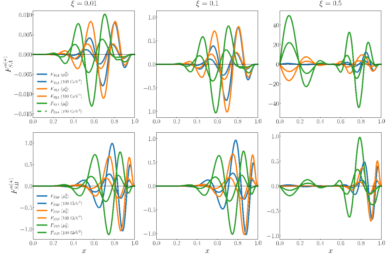
FIG. 2. Results for NLO SGPDs in the spin-independent quark sector. The top row shows three examples of type A SGPDs where the forward limit is maintained via constraints on the c_{mn} 's so that the SGPDs vanish as \xi \rightarrow 0 . In the second row, three type B SGPDs are illustrated where any forward-limit constraint is imposed via the unspecified t dependence. In each case, SGPDs with skewness \xi \propto 0.01; 0.1; 0.5 are shown in the panels from left to right. The SGPDs are defined at the input scale \mu_0 \propto 1.27 GeV (solid lines). These results are evolved at LO to \mu^2 \propto 100 GeV 2 (dotted lines), where these evolved results no longer satisfy the requirements for a SGPD.
