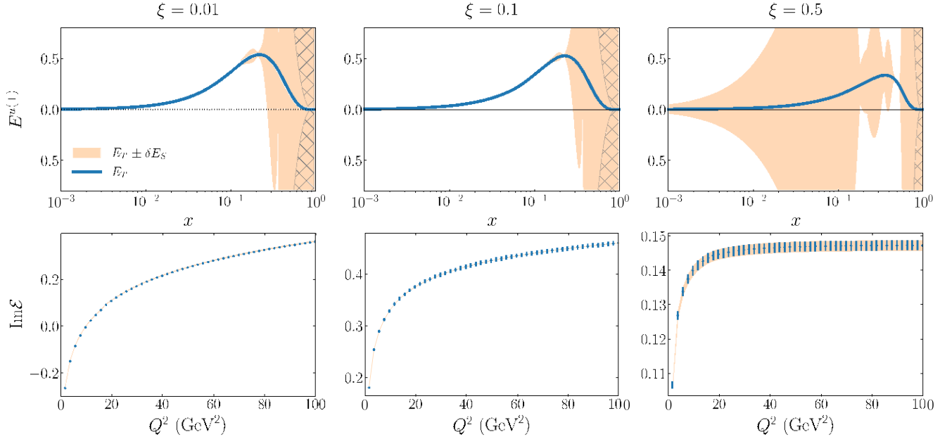
FIG. 4. Top row: results for the true GPD E_T^{u\delta bp} (blue lines) and the range of E_T^{u\delta bp} \pm \delta E_S (orange bands) at the input scale for three different values of \xi . The orange bands show the results for the three type B SGPDs in Fig. 2, appropriate for E^q GPDs because this is no forward limit constrain. The gray hashed region shows the area that would be excluded by the positivity constraint for E^q given in Eq. (23). Bottom row: simulated data (blue points) for the CFF \text{Im}E obtained using the VGG model GPDs with error bars showing 1% uncertainty, as a function of Q^2 , for fixed t , and three values of \xi . The light orange bands illustrate the 10000 sample CFFs associated with type B SGPDs.
