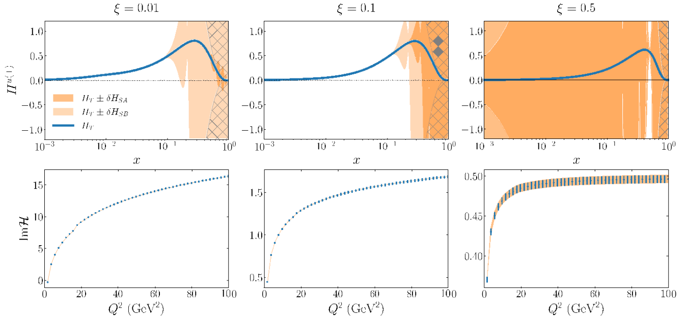
FIG. 3. Top row: results for the true GPD H_T^{u\delta\text{pp}} (blue lines) and the range of H_T^{u\delta\text{pp}} \pm \delta H_S (orange bands) at the input scale for three different values of \xi . The darker orange bands show the results for the three type A SGPDs in Fig. 2, while the lighter orange bands show the results for the type B SGPDs in Fig. 2. The gray hashed region shows the area that would be excluded by the positivity constraint for H^q given in Eq. (23). Bottom row: simulated data (blue points) for the CFF \text{Im}H obtained using the VGG model GPDs with error bars showing 1% uncertainty, as a function of Q^2 , for fixed t , and three values of \xi . The dark orange bands illustrate the 10000 sample CFFs associated with type A SGPDs.
