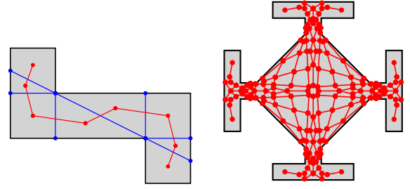
Fig. 9: Example position graphs, shown in red. Blue lines in the left example represent boundaries of the conservative regions.
