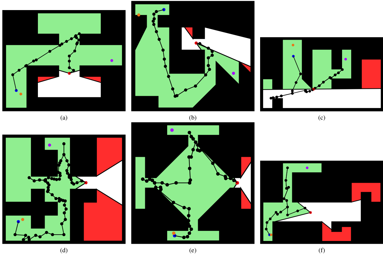
Fig. 10: Escort paths and final problem states computed by our algorithm in a variety of problem instances. Blue dots represent the starting positions of the escort, orange dots show the starting position of the VIP, red dots depict the end position of the escort, and purple dots mark the end/goal position for the VIP. The black lines depict the path taken by the escort. Green regions represent VIP-reachable safe zones. Red regions represent contaminated shadows.
