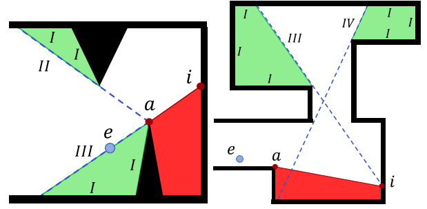
Fig. 7: Example environments illustrating the four types of safe zone boundary edges, determined by the escort’s position e and a shadow’s anchor point a and incident point i . Contaminated shadows are shown in red; safe zones are shown in green. [left] An environment with safe zone boundary edge Types I, II, and III. [right] An environment with safe zone boundary edge Types I, III, and IV.
