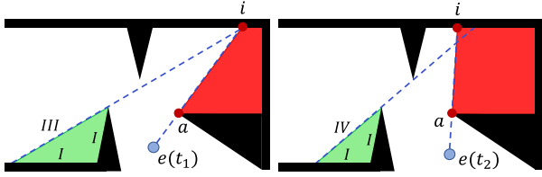
Fig. 8: Changes to the visibility polygon of the incident point of a shadow lead to changes in a safe zone.
