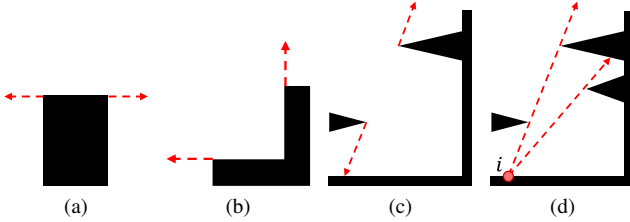
Fig. 6: Ray shooting methods to obtain conservative regions. Cases (a), (b), and (c) are part of the visibility cell decomposition used in many pursuit-evasion problems. Case (d) is a new case arising from potential changes in the safe zones for the VIP.
