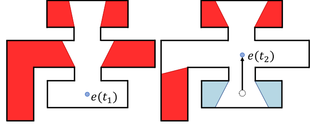
Fig. 2: [left] The initial state of shadows for the shown escort position e . There are four shadows, all contaminated, shown in red. [right] The shadows change after an upward movement by the escort. One shadow had disappeared and two new cleared shadows, shown in blue, have been created.
