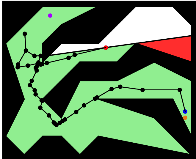
Fig. 1: An escort path, black line, which solves the escort problem. The blue dot is the escort’s starting position. The red dot is the escort’s end position. The orange dot is the VIP’s starting position. The purple dot is the VIP’s goal position. The green shaded region is a VIP-reachable safe zone. The red shaded region is a contaminated shadow.
