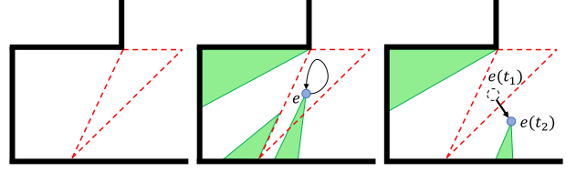
Fig. 4: [left] An example of a conservative region, shown by dashed red lines. [center] A path for the escort within the conservative region. The three safe zones, shown in green, are unaffected by this escort movement; each exists and is VIP-reachable before the movement and each remains VIP-reachable during and after the movement. [right] A movement for the escort that leaves a conservative region, creating a change in the safe zones. In this case, the middle safe zone disappears. If the escort were to return to the original position, that middle safe zone would reappear, but would be labeled as VIP-unreachable.
