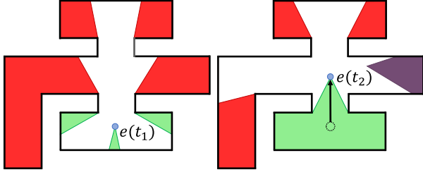
Fig. 3: A continuation of the example from Figure 2. Recall that after the escort’s upward movement, there are three contaminated shadows, shown in red. At this point, there are two safe zones: One shown in green which is VIP-reachable and another shown in purple which is VIP-unreachable. The two cleared shadows, which do not impact the safe zones, are not shown.
