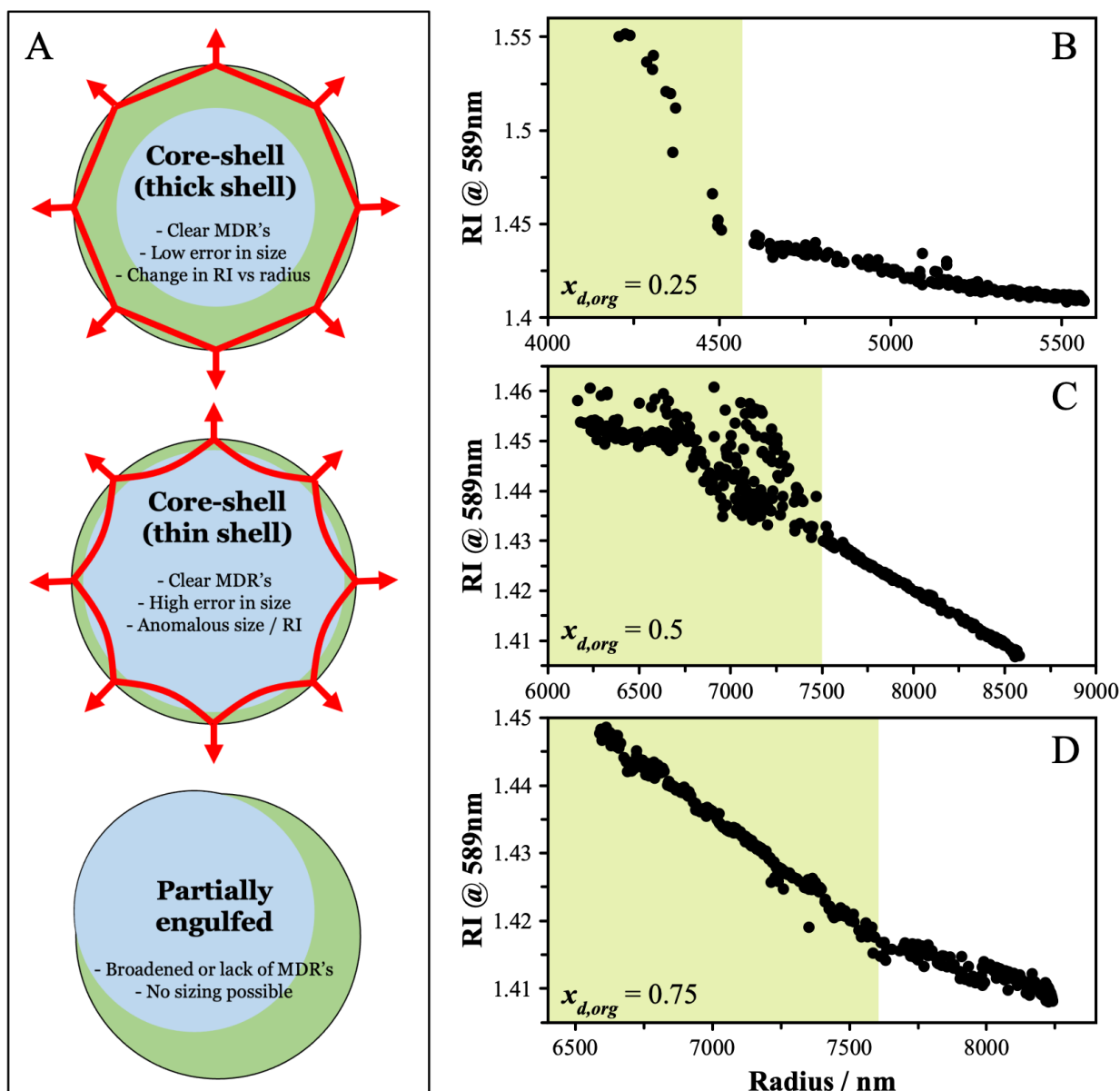
Figure 1: (A) Different morphologies will affect the MDR's and subsequent analysis, allowing LLPS to be identified. Green shading shows organic-rich regions and blue shading shown aqueous regions. (B) LLPS was identified in aqueous particles containing 3EG and AS from the discontinuity in the change in RI with radius as the RH was decreased, indicating core-shell morphologies with thick shells relative to the penetration depth of the MDR's (as shown in panel A – note that the position of the images in panel A do not correspond to the morphology observed in panels B-D). Three example starting particle compositions are shown, with dry organic mole fractions: (B) x_{d,org} = 0.25 ; (C) x_{d,org} = 0.5 ; and (D) x_{d,org} = 0.75 . In each panel, the shaded region indicates where the particle was liquid-liquid phase separated. Note these measurements are obtained by decreasing the RH continuously from a starting level of ~80% to 40% over a time span of around 2000 s.
