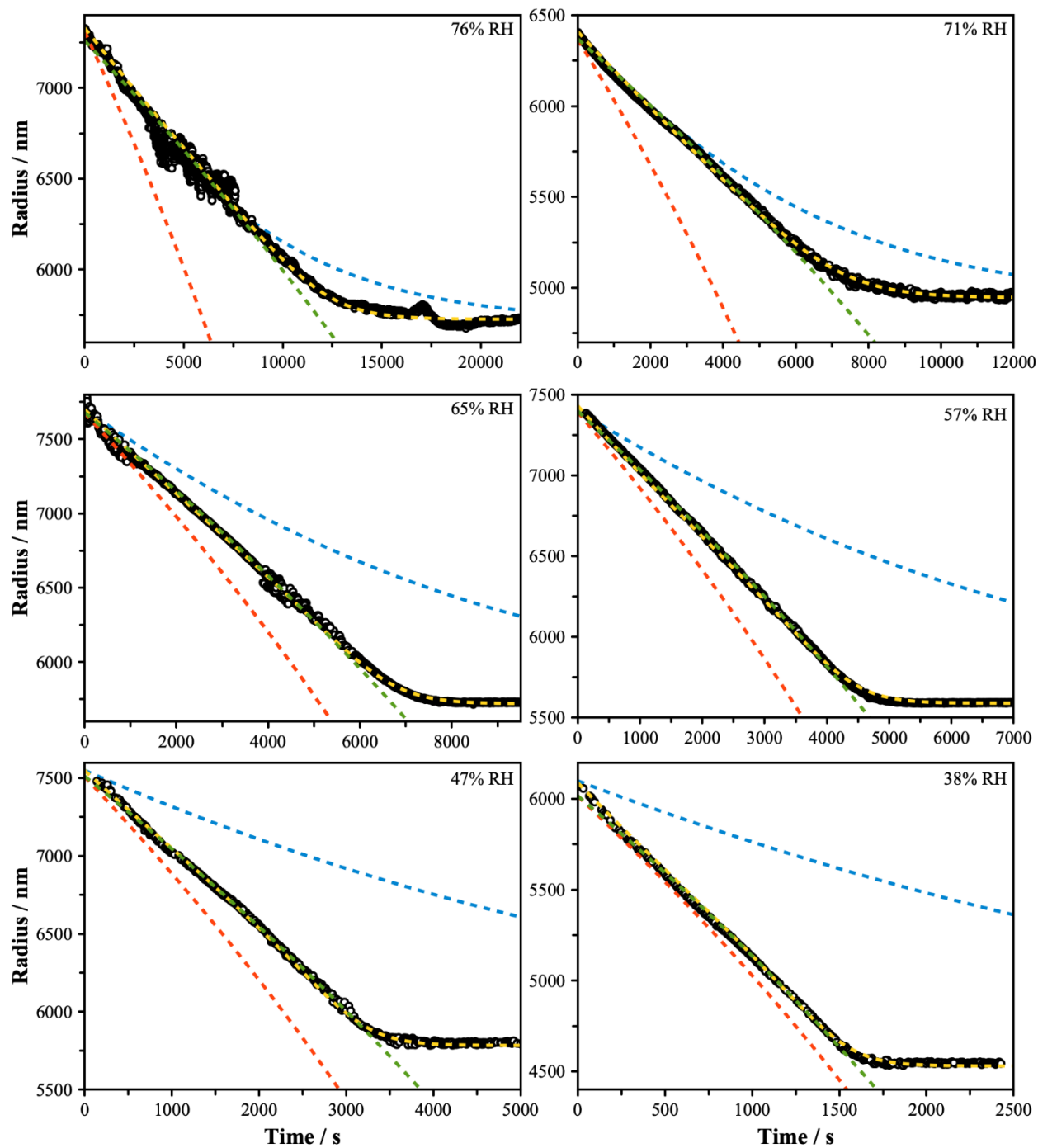
Figure 3: Evaporation measurements were performed over a range of RH conditions, as indicated, and span above and below the separation RH (~65%). In each panel, the blue dashed line shows the predicted trend assuming ideality (Model 1 – mole fraction scaled evaporation rates), the yellow dashed line assumes a well-mixed phase that exhibits non-ideality (Model 2), with fitted activity coefficients reported in Figure S4, and the red dashed line assumes a core-shell particle with a binary organic-rich shell (model 3). The green dashed line is a fit to a = (m t + a_0^2)^{0.5} , with radius a , starting radius a_0 and slope parameter m , equivalent to a linear fit of radius-squared versus time data for the early part of radius change measurements.
