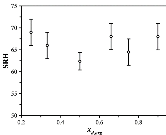
Figure 2: The separation RH (SRH) upon dehumidification at 293 K is shown as a function of the starting dry organic mole fraction ( x_{d,org} ) in the particle.
