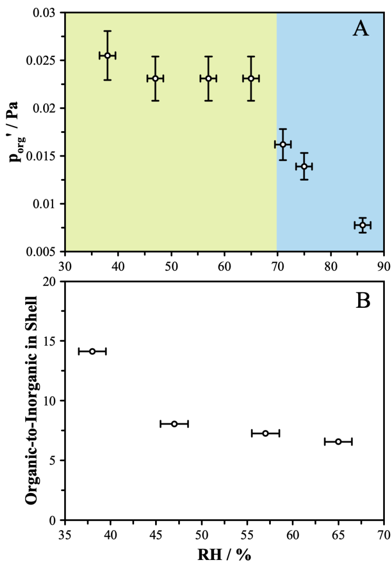
Figure 5: (A) Under the assumptions of core-shell behavior and an organic-rich phase that is modelled with a binary composition, the effective vapor pressure was determined from the slope of radius-squared versus time for the linear portion of the evaporation trajectories. The blue shaded region shows where the particle is assumed to be well-mixed (and thus this assumption fails) and the green shaded region shows where the particle is assumed to be phase-separated with a core-shell morphology. (B) In order to achieve closure between the pure-component vapor pressure and the expected vapor pressure, the organic-rich phase must include
