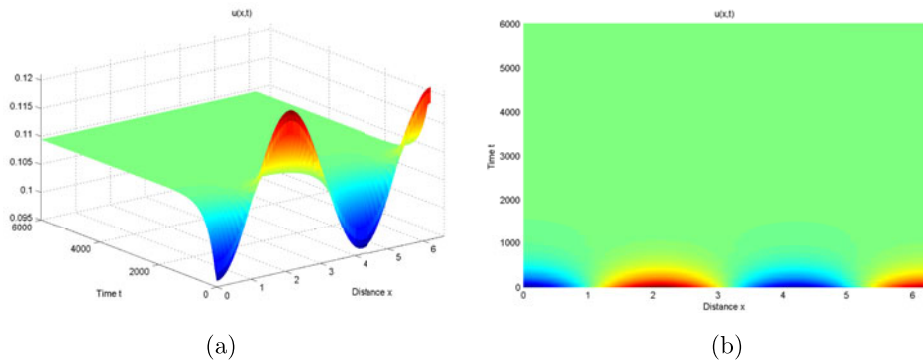
Figure 6. When (d_1, c) \in \text{I} in figure 5(a) for the (3, 0)-mode Turing–Hopf bifurcation, system (3.18) exhibits monostability: a positive constant steady state E_*(0.109, 1.629) .
