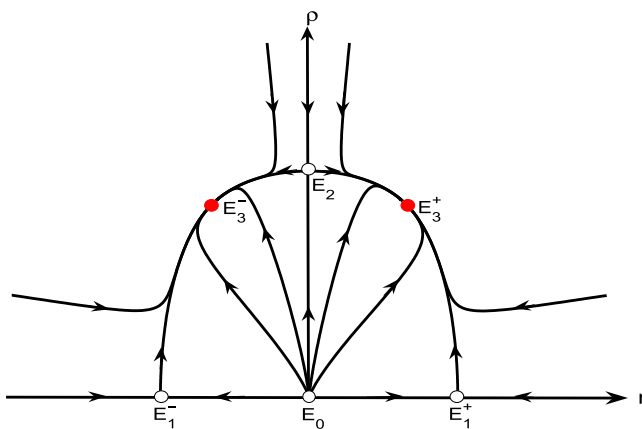
Figure 12. Phase portrait of system (3.26) for the (8, 0)-mode Turing–Hopf bifurcation when (\mu_1, \mu_2) \in \text{IV} in figure 5(a).
