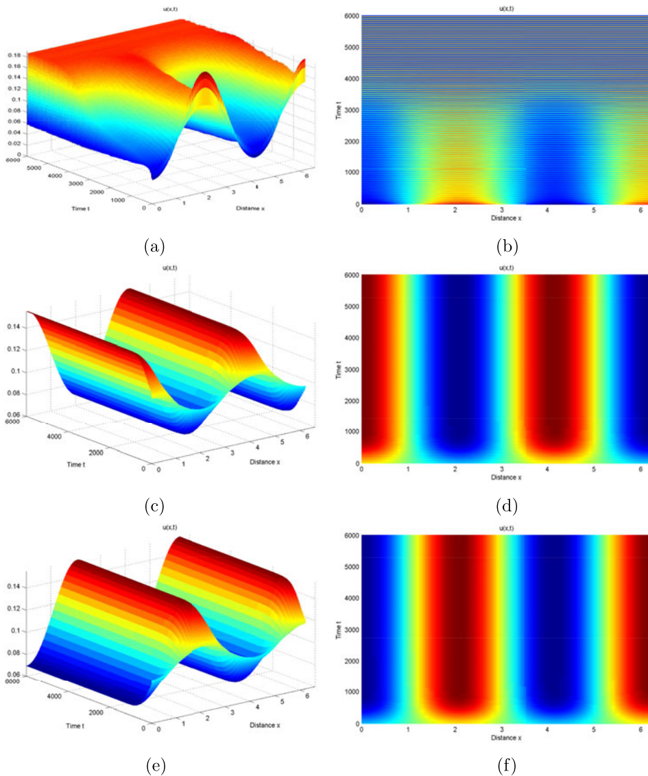
Figure 9. When (d_1, c) \in \text{IV} in figure 5(a) for the (3, 0) -mode Turing–Hopf bifurcation, system (3.18) exhibits a pair of unstable spatially nonhomogeneous periodic solutions and tristability: (a, b) transient spatially nonhomogeneous periodic solutions to a stable spatially homogeneous periodic solution, (c, d) one stable spatially nonhomogeneous steady state, and (e, f) the other stable spatially nonhomogeneous steady state.
