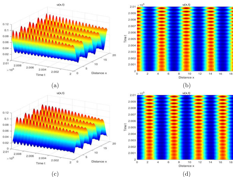
Figure 13. When (d_1, c) \in \text{IV} in figure 5(a) for the (8, 0) -mode Turing–Hopf bifurcation, a spatially homogeneous steady state, a pair of spatially nonhomogeneous steady states and a spatially homogeneous periodic solution are all unstable, while a pair of spatially nonhomogeneous periodic solutions is stable: (a, b) one stable spatially nonhomogeneous periodic solution, (c, d) the other stable spatially nonhomogeneous periodic solution, where u_0(x) = 0.05 \pm 0.03\cos(\frac{4}{3}x) , v_0(x) = 2.09 - 0.01\cos(\frac{4}{3}x) , (\mu_1, \mu_2) = (-0.001, -0.0006) .
