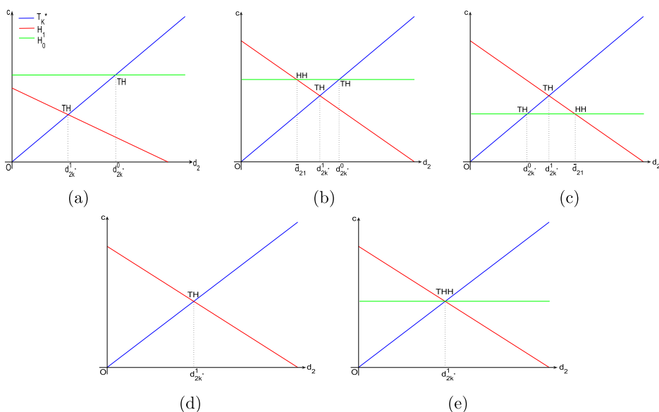
Figure 14. Turing–Hopf, double–Hopf, and Turing–double–Hopf bifurcations of system (1.3) near E_* in the (d_2, c) -plane for any l > 0 : (a) (a, b, e, u_*) \in U_{32} and u_* l^2 \leq d_1 < s_1 l^2 ; (b) (a, b, e, u_*) \in U_{32} , 0 < d_1 < u_* l^2 and d_{2k^*}^0 > \bar{d}_{21} ; (c) (a, b, e, u_*) \in U_{32} , 0 < d_1 < u_* l^2 and d_{2k^*}^0 < \bar{d}_{21} ; (d) (a, b, e, u_*) \in U_{31} ; (e) (a, b, e, u_*) \in U_{32} and d_{2k^*}^0 = \bar{d}_{21} . H_0 , H_1 , and T_{k^*} represent the 0-mode, 1-mode Hopf bifurcation, and k^* -mode Turing bifurcation curves, respectively. TH , HH , and THH represent Turing–Hopf bifurcation, double–Hopf bifurcation, and Turing–double–Hopf bifurcation, respectively.
