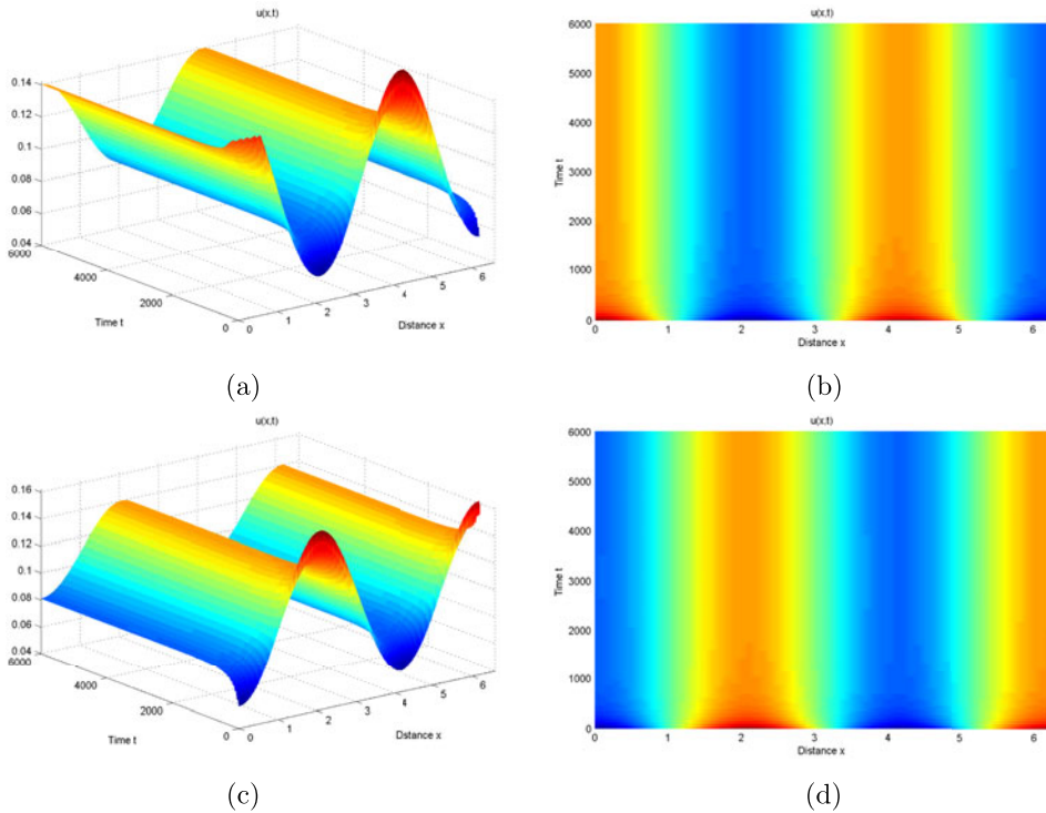
Figure 7. When (d_1, c) \in \text{II} in figure 5(a) for the (3, 0)-mode Turing–Hopf bifurcation, system (3.18) exhibits bistability: (a),(b) One spatially nonhomogeneous steady state and (c,d): the other spatially nonhomogeneous steady state.
