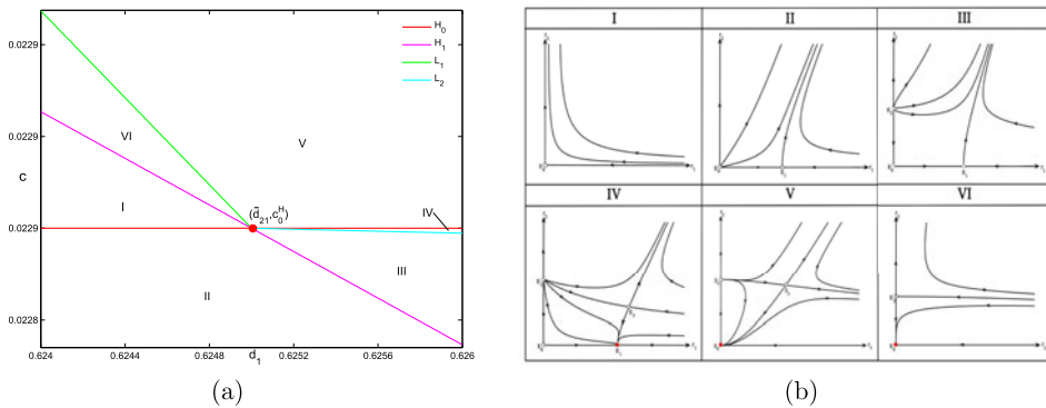
Figure 15. (a) Bifurcation set of system (4.26) near (\bar{d}_{21}, c_0^H) in the (d_2, c) -plane. (b) The corresponding phase portraits in I–VI, where H_0 , H_1 , L_1 , and L_2 represent critical bifurcation curves defined as in (4.27).
