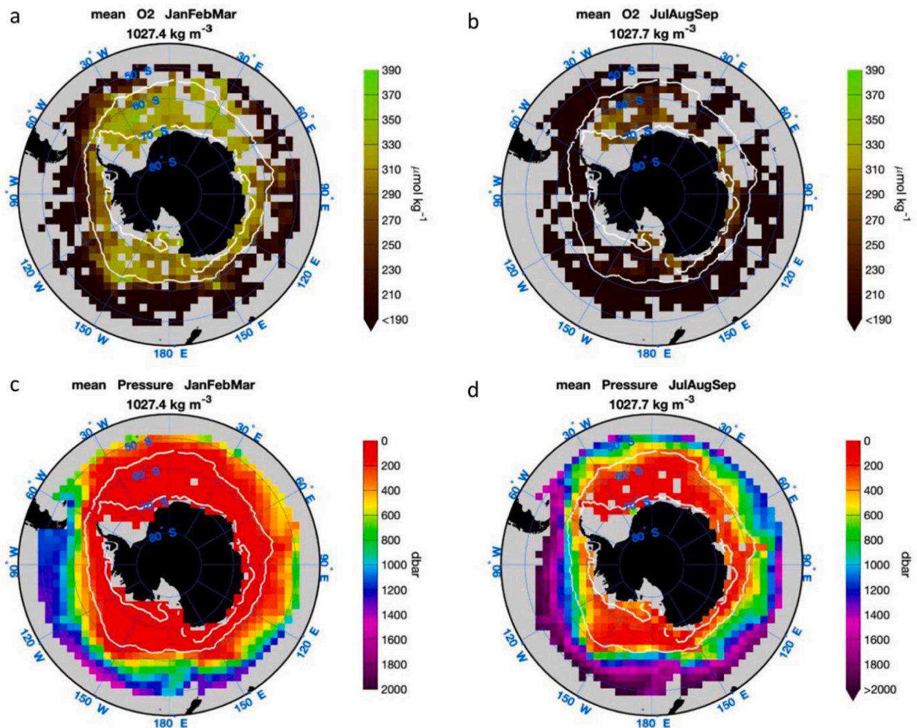
Fig. 15. Under ice climatology for oxygen. Dissolved O 2 (μmol kg -1 ) determined from SOCCOM float data in summer (panel a) and winter (panel b) on the pressure (decibars) surfaces shown in panels c ( \sigma_0 = 27.4 ) and d ( \sigma_0 = 27.7 ). These pressure surface lie at the base of the mixed layer in summer and winter and the O 2 concentrations represent values in the surface mixed layer. The inner and outer white contours represent the summer and winter limits of the sea ice zone. The climatologies are gridded using an equal area scalable Earth projection that preserves the gridding in cells near the pole.
