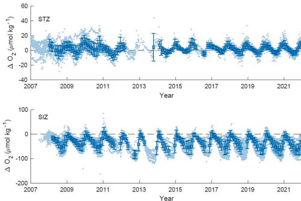
Fig. 8. Oxygen concentration difference from saturation ( \Delta\text{O}_2 = [\text{O}_2]_{\text{measured}} - [\text{O}_2]_{\text{saturation}} ) for the Subtropical Zone (STZ) and Sea ice Zone (SIZ). Updated from Bushinsky et al. (2017) with data through 2022. Light blue points indicate mixed layer concentrations from individual profile averages. Blue squares and error bars are monthly means \pm 1 \text{ SD} when average float temperature agreed with the NOAA Optimal Interpolation Sea Surface Temperature product as a check on data coverage.
