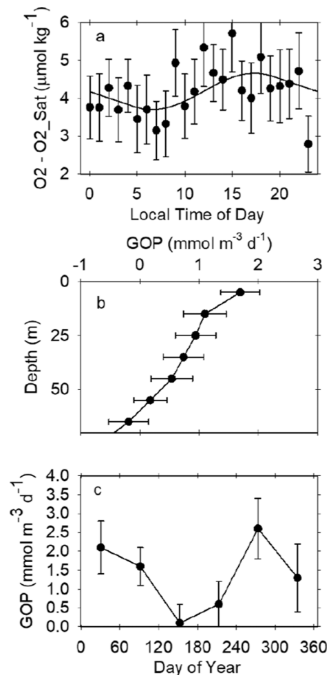
Fig. 12. Diel oxygen productivity from 30°S to 60°S following Johnson and Bif (2021). (a) Diel cycle of oxygen in the upper 20 m for all SOCCOM floats on days 0 to 61. (b) Vertical profile of Gross Oxygen Production (GOP). (c) Seasonal cycle of GOP in the upper 10 m. Error bars are 90% confidence intervals.
