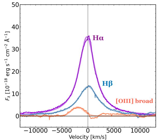
Fig. 8. Emission from the H\alpha and H\beta BLR lines and the [O III] \lambda 5007 broad component as a function of the velocity. Both the subtracted-data (solid lines) and the fitted models (semi-transparent thick curves) are shown. The systemic velocity, set by the vertical grey line, is based on the [C II] redshift. The H\alpha and H\beta lines are offset of a small amount compared to the zero-reference point ( \Delta v_{H\alpha} = -149 \pm 7 km s ^{-1} and \Delta v_{H\beta} = 87 \pm 15 km s ^{-1} ). On the other hand, we see that the [O III] \lambda 5007 broad component shows a velocity blueshift of \Delta v_{[\text{O III}]} = -1922 \pm 39 km s ^{-1} and a \text{FWHM}([\text{O III}]) = 2776^{+75}_{-74} km s ^{-1} . This blueshifted emission highlights possible outflowing material from the QSO host galaxy.
