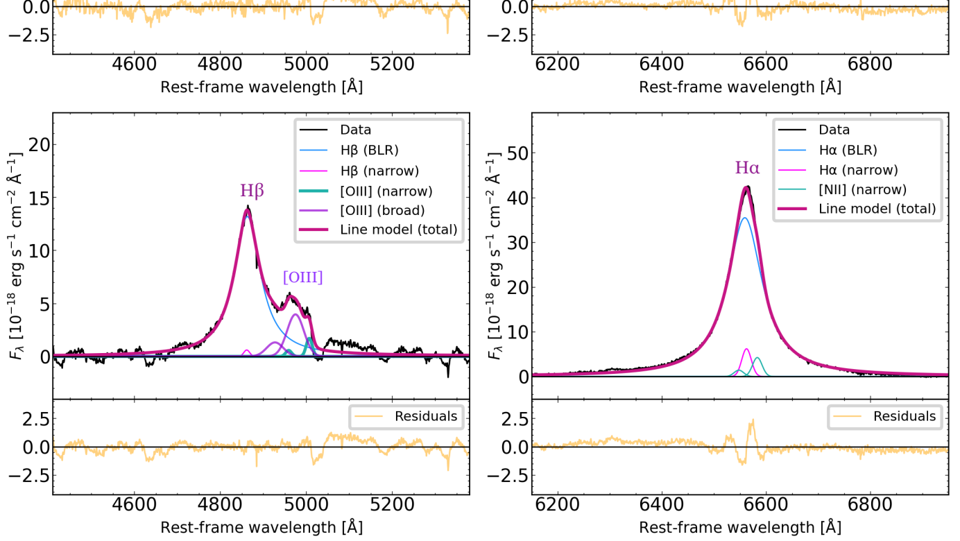
Fig. 5. Fit of the H \beta + [O III] ( left ) and H \alpha + [N II] ( right ), after the continuum and iron subtraction. We model the BLR H \beta and H \alpha lines using a Lorentzian function. The nebular lines from the NLR ([O III], [N II], H \alpha , H \beta narrow components) are each fitted with a Gaussian. We add two further Gaussian components (purple; "broad" components in the text) to fit the emission around 5000 Å, likely associated with blueshifted [O III] (see also Sect. 4.4 and Figure 8). The residuals are shown in orange.
