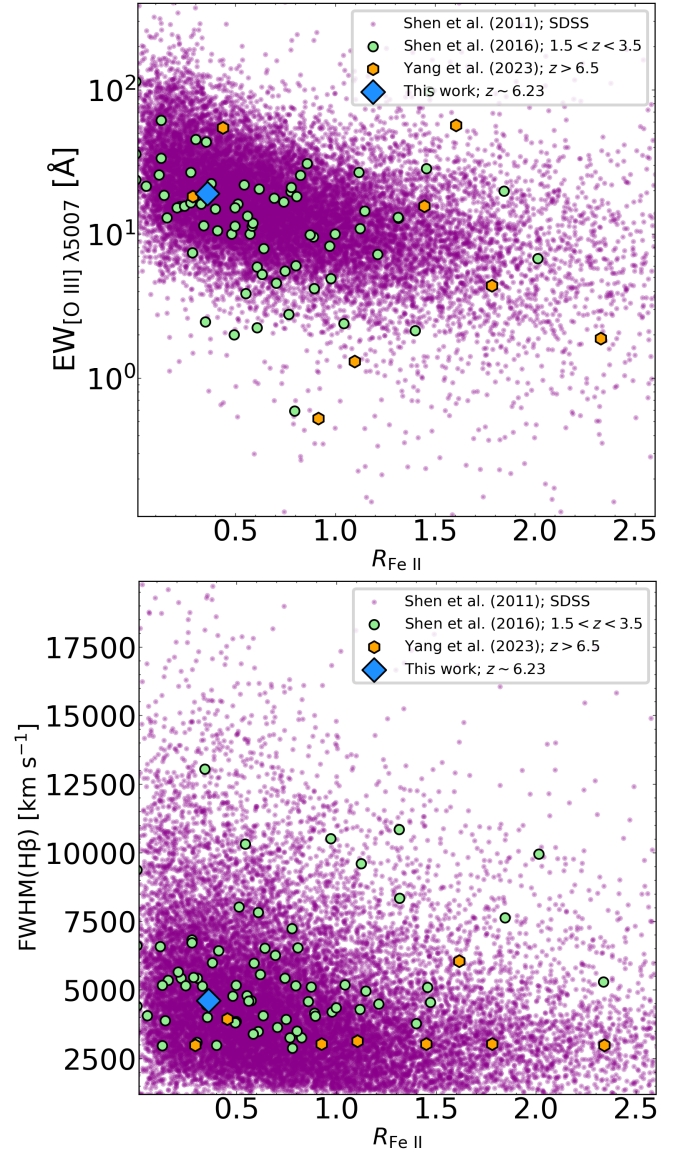
Fig. 7. Anti-correlations between the \text{Fe II} strength, parametrized by R_{\text{Fe II}} , the [\text{O III}] EW and \text{H}\beta FWHM. Top panel: the anti-correlation between R_{\text{Fe II}} and EW_{[\text{O III}]} (EV1 relation). PJ308-21 (blue diamond) shows a value in agreement with both low-redshift (Shen et al. 2011), 1.5 < z < 3.5 (Shen 2016) and z > 6 quasars (Yang et al. 2023). Bottom panel: anti-correlation between R_{\text{Fe II}} and \text{FWHM}(\text{H}\beta) (2D EV1). Also in this case, the PJ308-21 value appears consistent with the findings of other studies.
