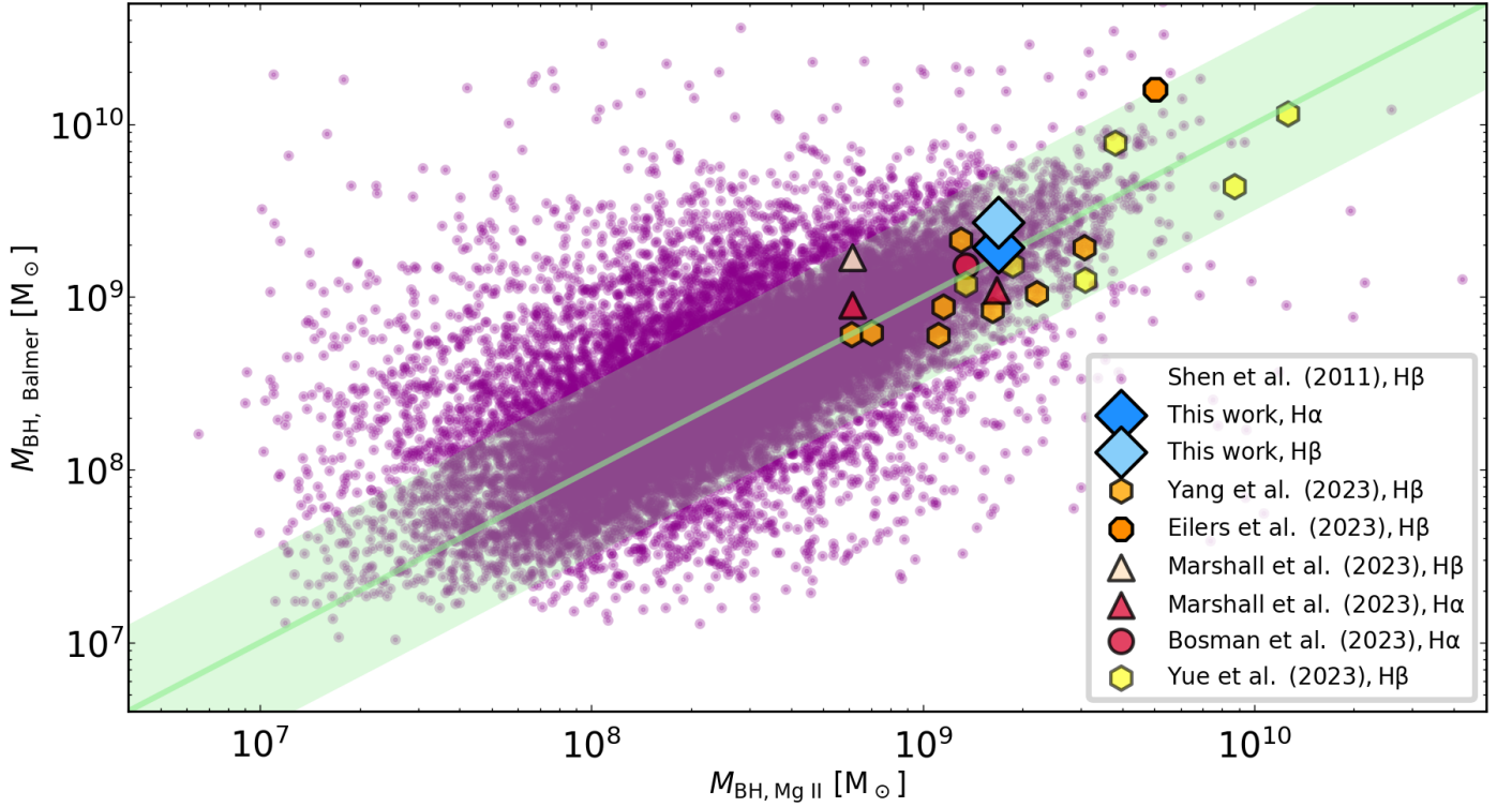
Fig. 6. Black hole masses from SDSS (Shen et al. 2011) and z > 6 quasars (Bosman et al. 2023; Eilers et al. 2023; Marshall et al. 2023; Yang et al. 2023; Yue et al. 2023), with both Mg II and Balmer line based measurements. The green line shows the one-to-one relation. PJ308-21 is indicated with blue diamonds (JWST/NIRSpec and VLT/XSHOOTER data). Overall, the z > 6 quasars show nice agreement between the Mg II and H \beta or H \alpha -based M_{\text{BH}} , consistent with the \sim 0.5 dex scatter of the low-redshift estimates (green region; Vestergaard & Peterson 2006). While a larger sample is needed to confirm these results, these first JWST estimates suggest that the Mg II is a reliable tracer of the black hole mass at both low and high-redshift.
