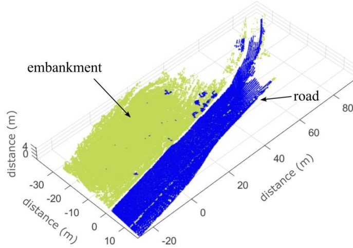
Figure 4: Segmentation of road and embankment through analysis of normal vectors and curvature values of each point in the point cloud, distinguishing between the road (blue) and bank (green) regions.
