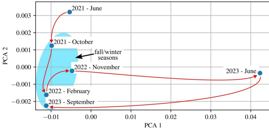
Figure 5: Results for the curvature embedding via PCA with two principal components.
