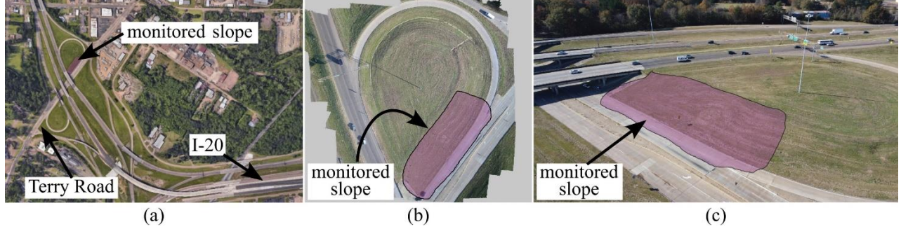
Figure 1: Monitored earthen embankment located at the I-20 East exit onto Terry Road in Jackson Mississippi, showing: (a) a satellite view of the reference slope (base image credit Google Earth), (b) a composite image obtained from UAV flights at the test location, and; (c) a UAV image taken from the North-East side of the slope.
