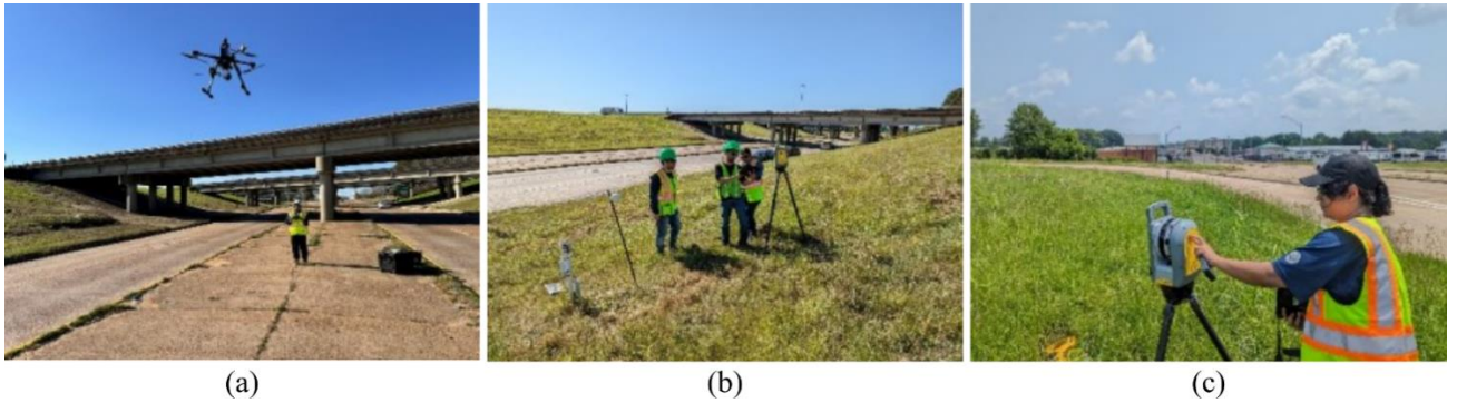
Figure 2: Field data collection, showing the data collection crew: (a) operating the UAV used to obtain aerial footage of the slope; (b) LiDAR set up on the slope, and; (c) LiDAR scanner during operation.
