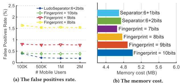
Figure 11: Evaluation of Ludo Separator against locator-only approaches.
