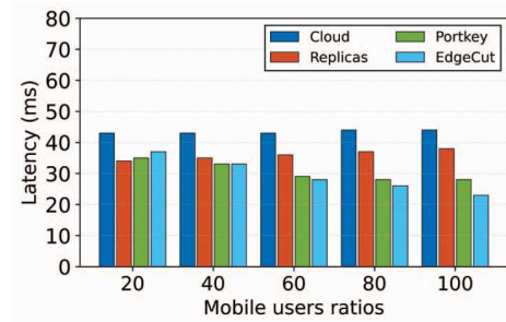
(b) Average latency of accessing user-associated content.
