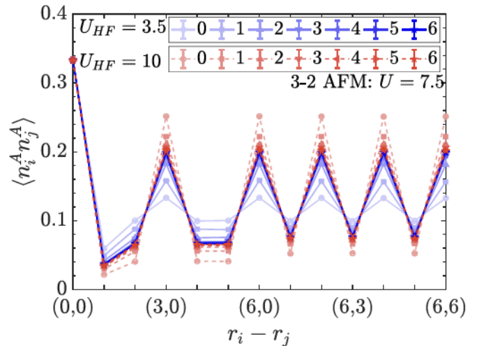
FIG. 5. Illustration of convergence of real-space density-density correlation. We have chosen U_{c1} < U = 7.5 < U_{c2} , where the system is in the 3-2 AF phase. Spin correlations converge from lower and higher values when the starting point is in the 3-2 phase using an initial Slater determinant with U_{\text{eff}} = 3.5 and 10, respectively. The legend indicates the number of self-consistent iterations.
