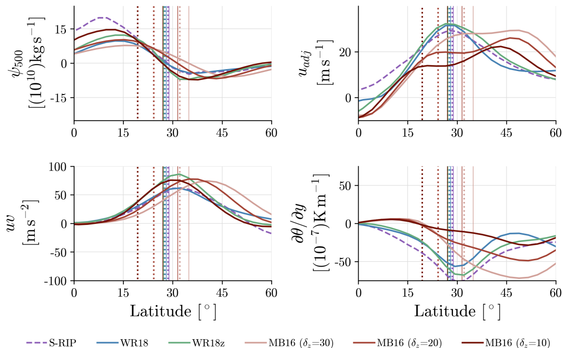
Figure 5. NH DJF zonal-mean meridional streamfunction at 500 hPa (top left), adjusted wind (top right), vertically averaged eddy momentum flux between 200–400 hPa (bottom left), and vertically averaged meridional temperature gradient between 100–400 hPa (bottom right) for S-RIP, WR18, WR18z, MB16 (default, \delta_z = 10 ), MB16 ( \delta_z = 20 ), and MB16 ( \delta_z = 30 ). The dotted and solid thin vertical lines show the climatological \phi_{STJ} and climatological \phi_{HC} , respectively, for each corresponding simulation.
