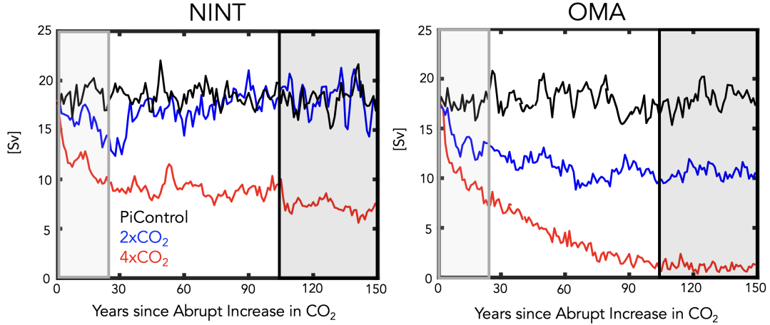
FIG. 2. Evolution of the annual mean maximum overturning stream function in the Atlantic ocean, evaluated at 48°N, for the preindustrial control (black), abrupt 2xCO 2 (blue) and abrupt 4xCO 2 (red) simulations. Results for the NINT (left) and OMA (right) configurations are shown. Light grey and black shaded boxes denote the “fast” and “total” timescale response averaging periods.
