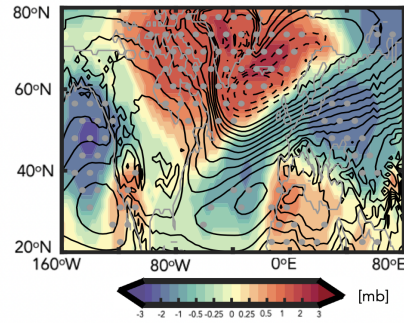
FIG. A3. Top panel: Colors show the LINOZ minus NINT ensemble mean difference in the December-January-February (DJF) “fast” response of the sea level pressure to an abrupt quadrupling of CO 2 . Results are shown for the fully coupled atmosphere-ocean simulations. Bottom panel: The ensemble mean response in sea level pressure in the experiments in which the time-evolving 4xCO 2 ensemble mean LINOZ ozone response is prescribed and the SSTs, SICs, and background CO 2 are set to preindustrial values. Black contours denote climatological mean preindustrial control DJF values (contour interval: 10 mb). Stippled regions are statistically significant.
