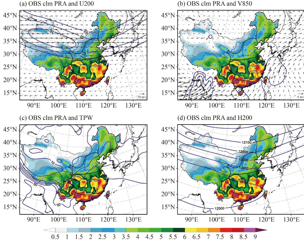
Fig. 3 Geographic distributions of 1980–2015 mean observed summer precipitation (PRA, mm·day -1 ), overlaid with ERA5 (a) 200-hPa wind vectors and zonal wind (U200, contours at 5 m·s -1 intervals starting from 20), (b) 850-hPa wind vectors and meridional wind (V850, contours at 1 m·s -1 intervals starting from 3), (c) total precipitable water (TPW, 10 mm contour intervals), and (d) 200-hPa geopotential height (H200, 100 gpm contour intervals).
