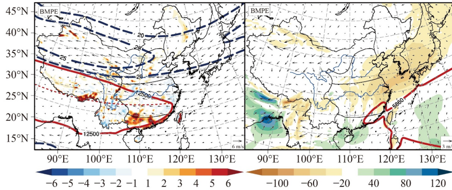
Fig. 15 CWRf BMPE simulated (left) summer mean 200-hPa wind ( \text{m}\cdot\text{s}^{-1} , vectors) departures from ERA5, overlaid with precipitation biases (color shadings), 200-hPa wind speeds ( \text{m}\cdot\text{s}^{-1} , dashed contours starting from 20 at intervals of 5), and 200-hPa geopotential height (solid contour at 12500 gpm with ridge as red dash contour). (right) 850-hPa wind ( \text{m}\cdot\text{s}^{-1} , vectors) and vertically integrated (1000–300 hPa) moisture flux ( \text{kg}\cdot\text{m}^{-1}\cdot\text{s}^{-1} , color shadings) departures from ERA5, overlaid with the 500-hPa geopotential height represented by solid contour at 5860 gpm.
