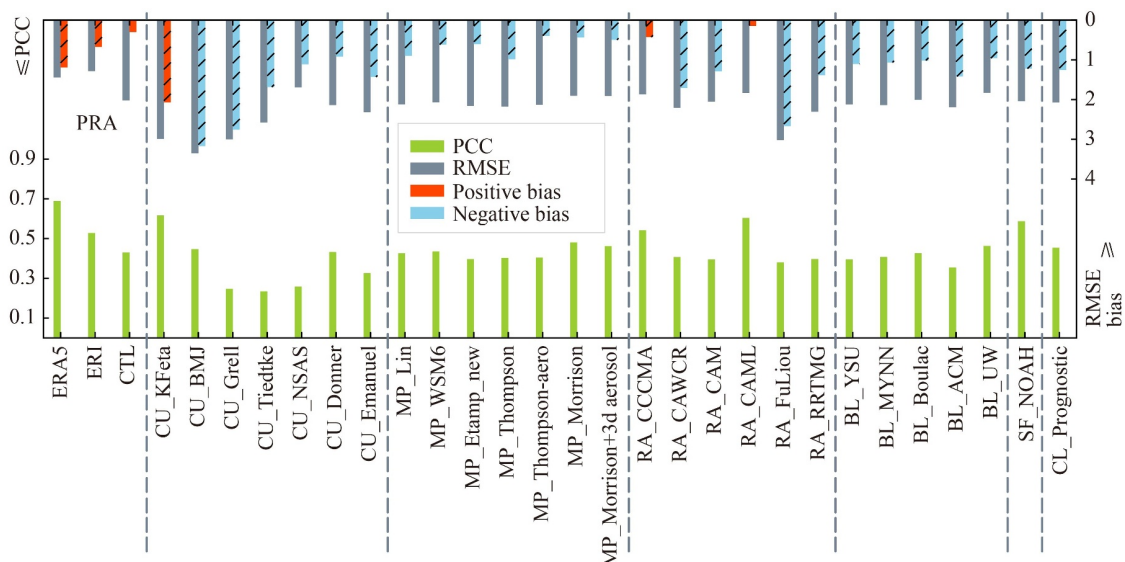
Fig. 1 The spatial pattern correlation coefficient (PCC), RMS error (RMSE), and average bias (Bias) between observations and ERA5, ERI, and 28 CWRf physics configurations for 1980–2015 mean summer precipitation (PRA, mm·day -1 ) over the YRB. Hatches denote statistically significant differences at the 5% significance level.
