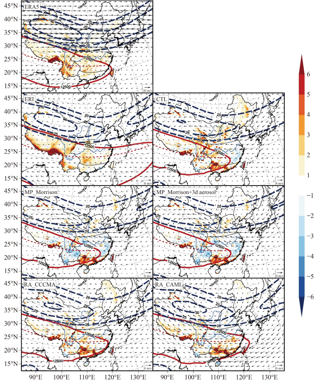
Fig. 10 1980–2015 mean summer wind at 200 hPa ( \text{m}\cdot\text{s}^{-1} , vectors) based on ERA5 and their departures from ERA5 as indicated by ERI and five CWRP physics configurations. Overlaid are the corresponding precipitation biases (from observations, color shadings), 200-hPa wind speeds ( \text{m}\cdot\text{s}^{-1} , dashed contours starting from 20 at intervals of 5), and 200-hPa geopotential height represented by solid contour at 12,500 gpm with its ridge (red dash contour).
