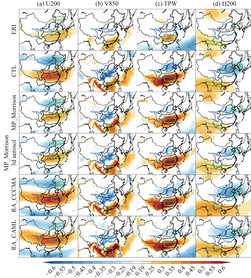
Fig. 12 Same as Fig. 5 except for interannual correlations of ERI and five CWRf physics configurations.
