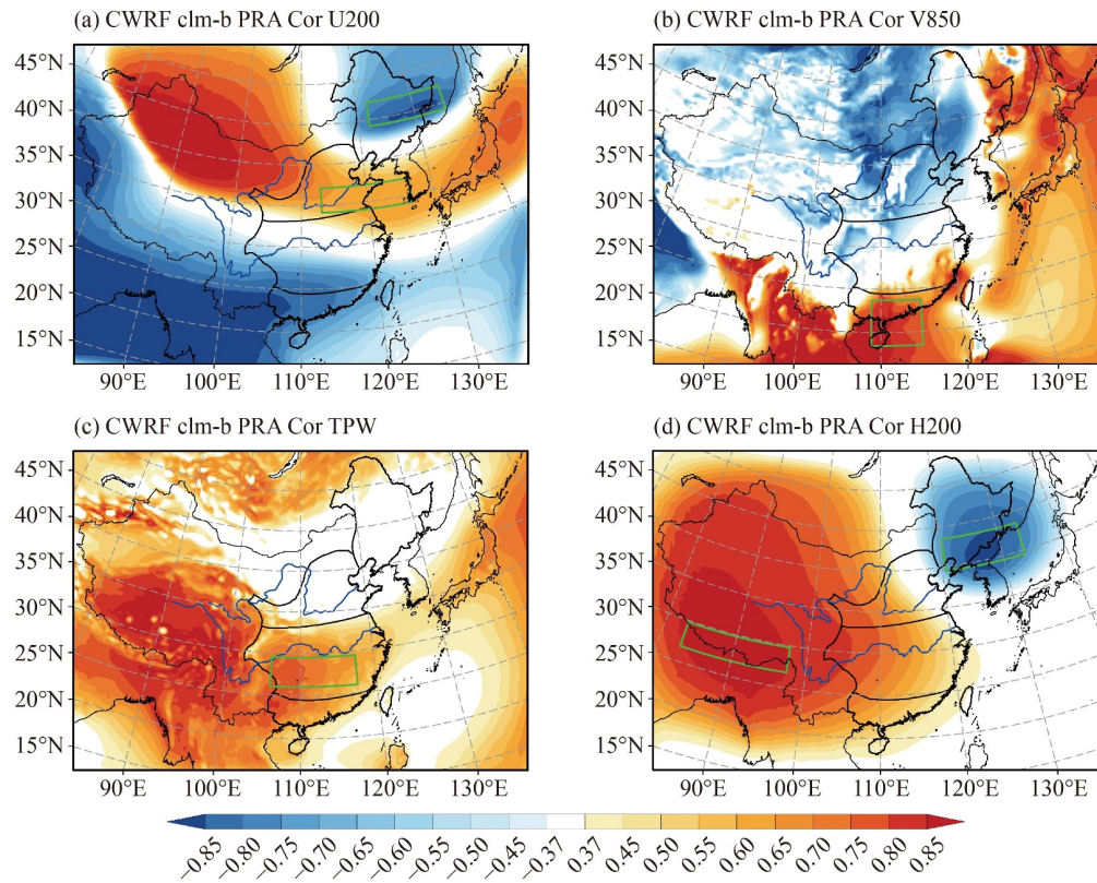
Fig. 4 Spatial distribution of correlations between long-term mean YRB-average summer precipitation biases (from observations) among ERI and 28 CWRf physics configurations, and their pointwise circulation departures (from ERA5) for (a) U200, (b) V850, (c) TPW, and (d) H200. Colored areas indicate statistically significant correlations at the 5% significance level, assuming individual model independence. The outlined regions with statistically significant high (positive or negative) correlations are defined as the core correlation areas, which are used to compute the circulation bias indices.
