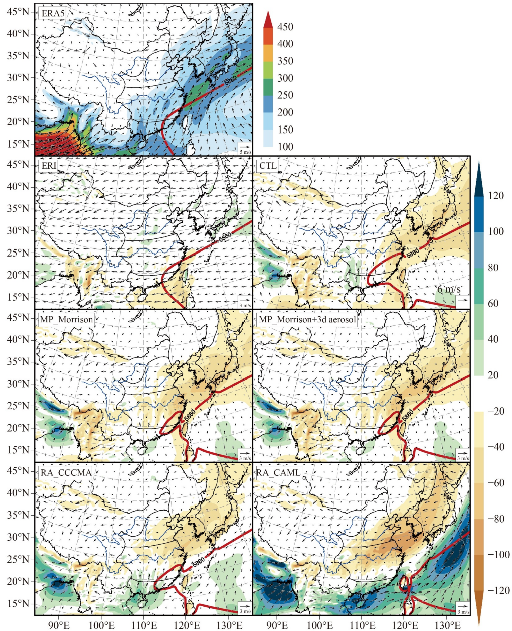
Fig. 11 1980–2015 mean summer wind at 850 hPa ( \text{m}\cdot\text{s}^{-1} , vectors) and vertically integrated (1000–300 hPa) moisture flux ( \text{kg}\cdot\text{m}^{-1}\cdot\text{s}^{-1} , color shadings) based on ERA5 and their departures from ERA5 as indicated by ERI and five CWFV physics configurations. Overlaid are the corresponding 500-hPa geopotential height represented by solid contour at 5860 gpm.
