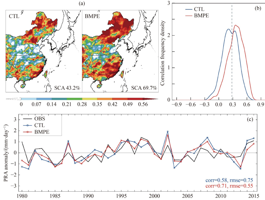
Fig. 14 CWRf CTL and BMPE simulated (a) interannual correlations of summer precipitation with observations, along with the percentage of basin areas that have significant interannual correlations (SCA). (b) frequency density functions of correlations at all CWRf grids within the YRB. Correlations above 0.28 marked by the vertical line are statistically significant at the 5% significance level, determined by a one-tail Student's t -test. (c) YRB-average precipitation interannual anomalies, along with their interannual correlation (corr) and RMS error (rmse) against observations.
