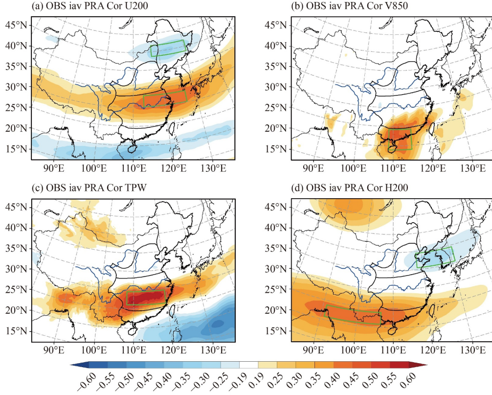
Fig. 5 Spatial distribution of correlations between the interannual anomalies of the observed YRB-average summer monthly precipitation and those of the ERA5 pointwise circulation for (a) U200, (b) V850, (c) TPW, and (d) H200. Colored areas denote statistically significant correlations at the 5% significance level, assuming monthly independence. The outlined regions with statistically significant high (positive or negative) correlations are defined as the core correlation areas, which are used to compute the circulation indices.
