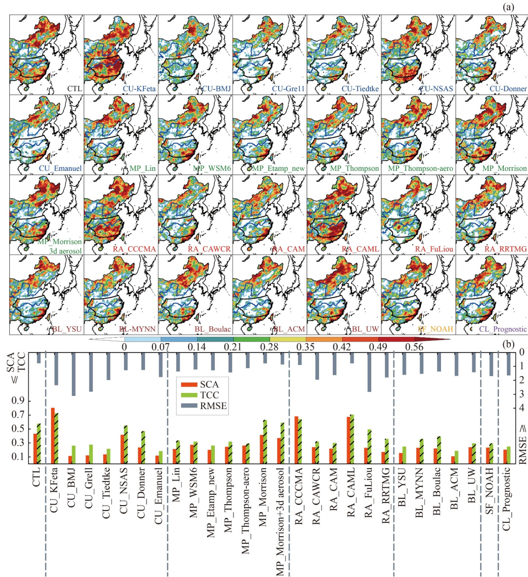
Fig. 2 (a) Geographic distributions of 1980–2015 summer precipitation interannual correlations between observations and 28 CWRf physics configurations. (b) YRB-average temporal correlation coefficient (TCC) and RMS error (RMSE, mm·day -1 ), and the percentage of areas in the YRB that have significant interannual correlations (SCA × 100, %). Correlations exceeding 0.28 as column hatched denote the 5% significance level under the one-tail Student's t -test. The YRB region is enclosed by the thick black outline.
