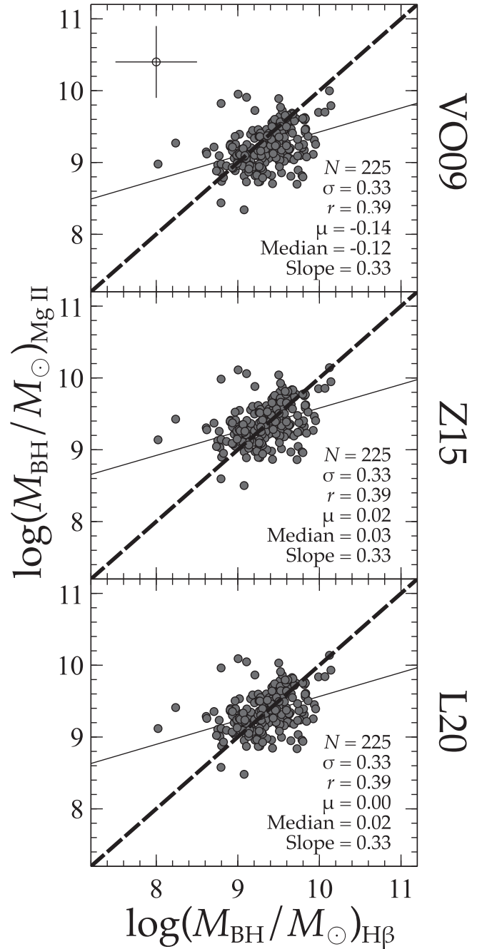
Figure 8. \text{Mg II} -based M_{\text{BH}} estimates of our sample derived through the methodology of, from top to bottom, VO09 , Z15 , and L20 against the \text{H}\beta -based M_{\text{BH}} estimates. The panels include all \text{Mg II} measurements available in SDSS and/or GNIRS. The dashed line in each panel represents a one-to-one relationship, and the thin solid line in each panel represents the best linear fit to the data. We find that our results are consistent with those of previous work when only measuring \text{Mg II} but are clearly improved with the inclusion of the C IV EW term (see the leftmost panels of Figure 6). Our prescriptions, by design, correct the mean offsets (the \mu value in each panel) between the \text{Mg II} - and \text{H}\beta -based M_{\text{BH}} values with or without the inclusion of the C IV EW. Typical uncertainty of 0.5 dex on the M_{\text{BH}} values is displayed in the top panel for reference.
