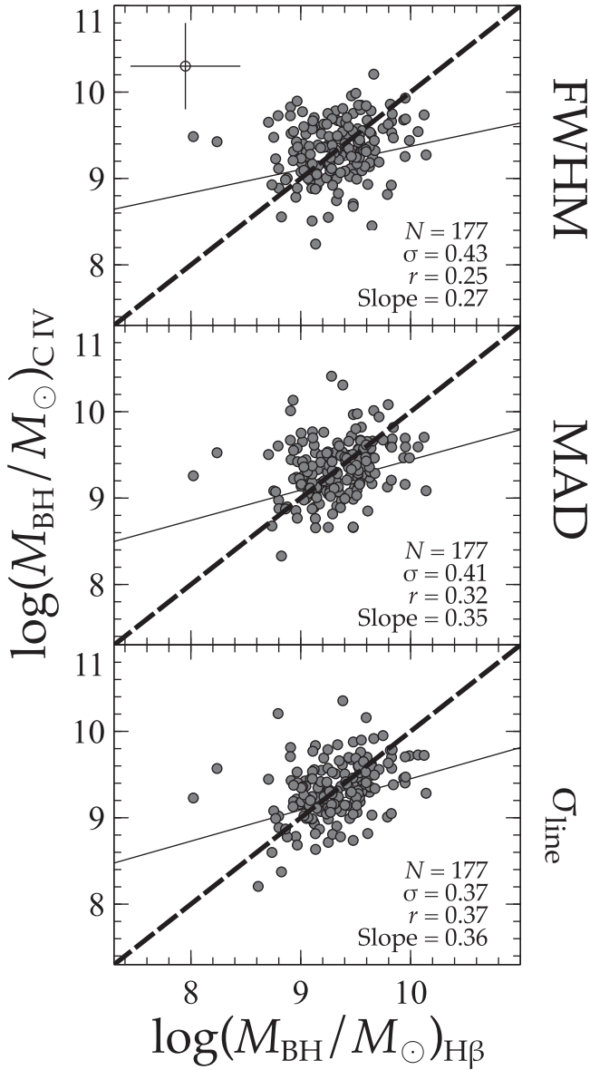
Figure 2. The calibrated C IV-based M_{\text{BH}} estimates using the three velocity width parameters, discussed in Section 3.1, against the calibration set of H \beta -based M_{\text{BH}} estimates. The dashed line in each panel represents a one-to-one relationship, and the thin solid line in each panel represents the best linear fit to the data. The Pearson correlation coefficient ( r ) and the slope of the best-fit line are provided in each panel. Notably, using \sigma_{\text{line}} as the velocity width parameter provides the most precise C IV-based M_{\text{BH}} estimates with respect to the H \beta -based M_{\text{BH}} estimates. Additionally, using \sigma_{\text{line}} as the velocity width parameter leads to the largest Pearson correlation coefficient and steepest slope of the best-fit relation. Typical uncertainty of 0.5 dex on the M_{\text{BH}} values is displayed in the top panel for reference.
