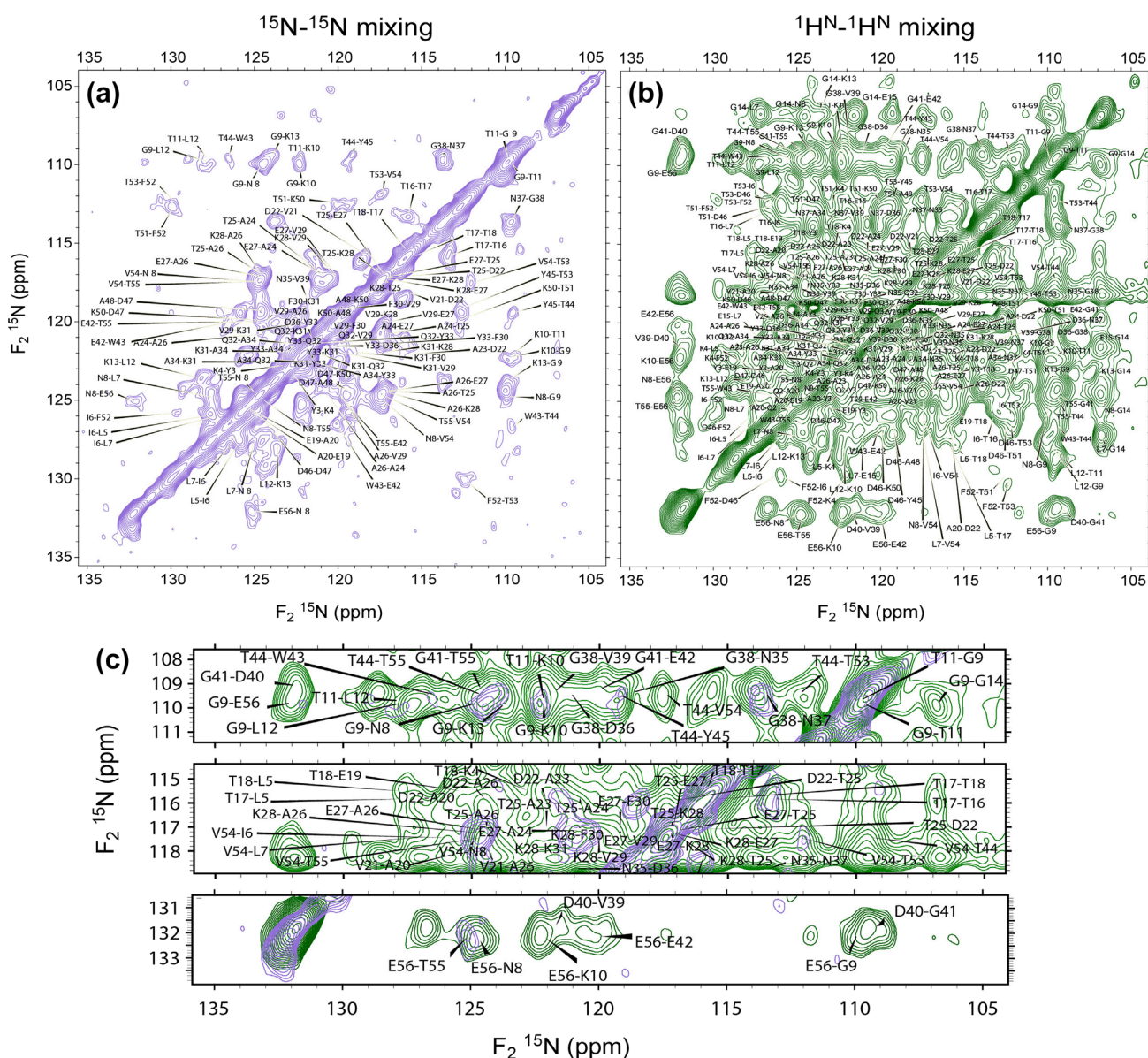
Fig. 3 Peak assignments and comparisons between the ^{15}\text{N} – ^{15}\text{N} correlation spectra obtained a by the direct ^{15}\text{N} – ^{15}\text{N} AL FRESKO, and b by the indirect ^1\text{H} – ^1\text{H} AL FRESKO scheme. The spectrum shown in a is identical to that shown in the second row of Fig. 1c and the
