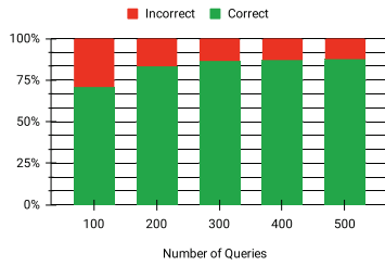
(a) Add-Remove Set (js-delta-crds)
