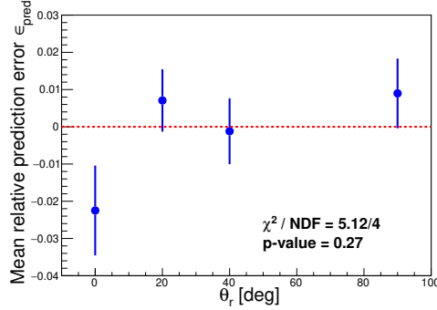
Figure 1. Mean relative prediction error for each \epsilon_{pred} distribution obtained by splitting data into the four angular datasets. The red dashed line marks the \epsilon_{pred} = 0 level (no directional effect).
