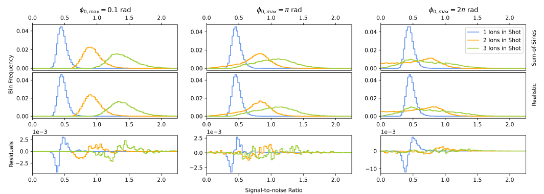
Figure 4. A comparison of the signal-to-noise (SNR) ratio distributions for N = 1, 2, 3 ions in the SIPT. Three different phase spread distributions are investigated, with each plot comparing the ‘sum of sines’ approach ( top ) of Equation (11) to the rigorous method of [9] ( middle ), and the residuals between the two methods ( bottom ). For each ion number, 10^4 simulated signals make up each distribution.
