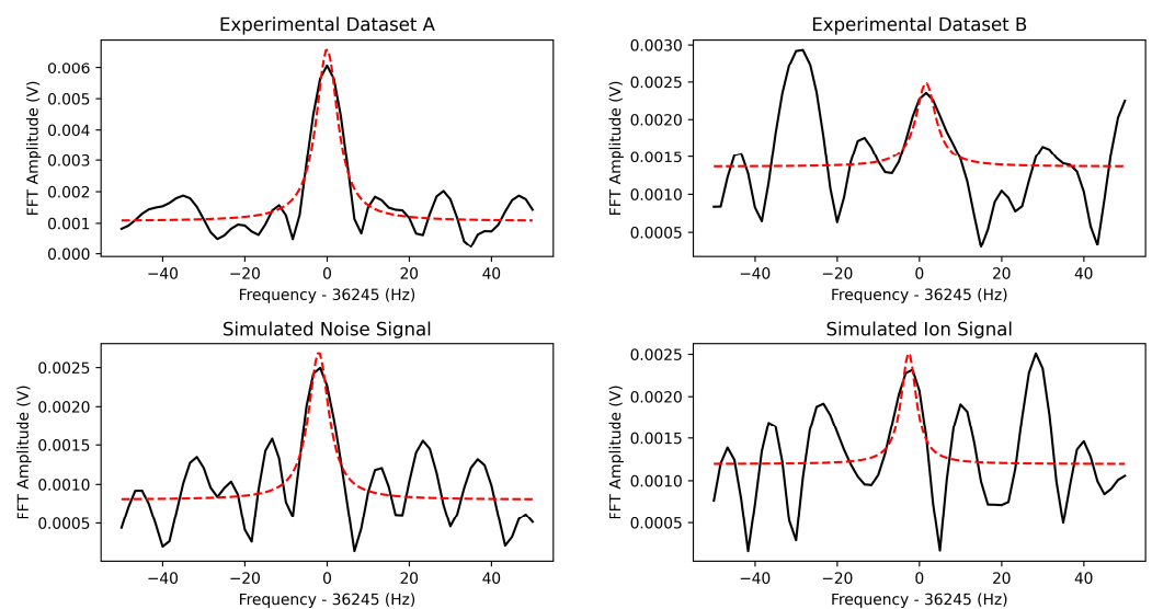
Figure 1. Frequency spectra for Fourier transform ion cyclotron resonance signals from the single-ion Penning trap (SIPT) for various measured and simulated ^{85}\text{Rb}^+ ion signals. The black line indicates the experimental dataset, the dashed red line shows one possible Lorentzian distribution fit to the dataset. Top Left: Example of a measured SIPT signal, likely from real ions, easily distinguished from noise as a strong peak is present near the expected frequency. Top Right: A measured signal which is ambiguous as the identified peak frequency may also just be noise. Bottom Left: Example of a simulated noise signal which exhibits a strong peak near the expected frequency, easily mistaken for a signal produced by an ion. Bottom Right: A simulated signal created by two ions whose peak frequency is easily mistaken for noise due to destructive interference.
