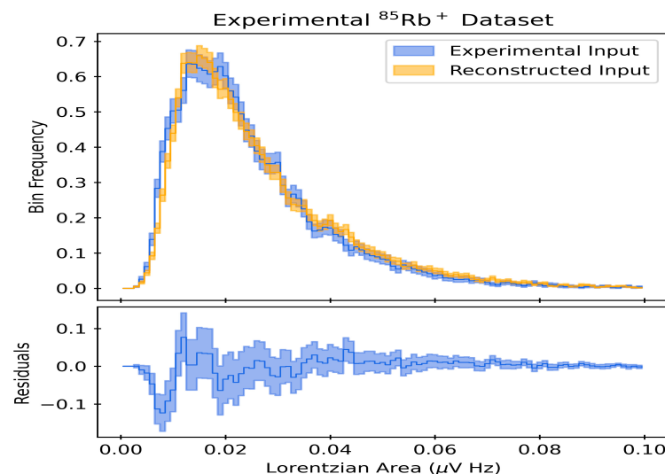
Figure 8. Comparison of a histogram of experimental ^{85}\text{Rb}^+ SIPT signal Lorentzian areas (defined by Equation (6)) to a histogram of 80,000 simulated ^{85}\text{Rb}^+ SIPT signals which was generated from the parameters predicted by the neural network; summarized in Table 3. Small residuals correspond to both reasonable predictions from the neural network as well as reasonable simulations of the SIPT FT-ICR signals.
