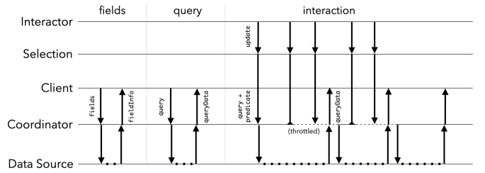
Fig. 3: Example Mosaic event timeline (not to scale). A client can provide a list of fields for which the Coordinator returns metadata. Next, the Coordinator requests a query from the Client, submits it to a Data Source for execution (dotted lines), and returns the result, providing the data the client needs to render. Interactions such as interval selections or pan/zoom update the state of linked Params or Selections , triggering additional rounds of query and update. While a query is being executed, corresponding selection updates are throttled (dashed lines): intermediate updates are dropped and only the most recent update is serviced.
