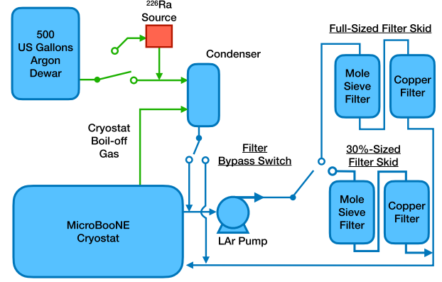
FIG. 1. The MicroBooNE cryogenic circulation system, including the modifications made to include a ^{226}\text{Ra} source inline with the flow of new liquid argon for special R&D periods described in this analysis. Gaseous and liquid argon flow is represented by green and blue lines, respectively, with arrows indicating the direction of flow. A filter bypass switch enabled a special flow configuration in which recondensed argon flowed directly into the cryostat without first passing through the filters. A second switch following the LAr pump determined whether circulating LAr flowed through the full-sized filter skid or the smaller 30%-sized filter skid [44].
