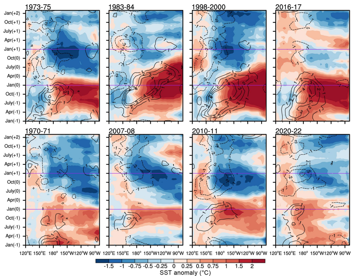
Extended Data Fig. 3 | Evolution of each multiyear La Niña event during the post-1970 period. SST (shading, °C) and 1000hPa zonal wind (contours, m s -1 ) anomalies.
