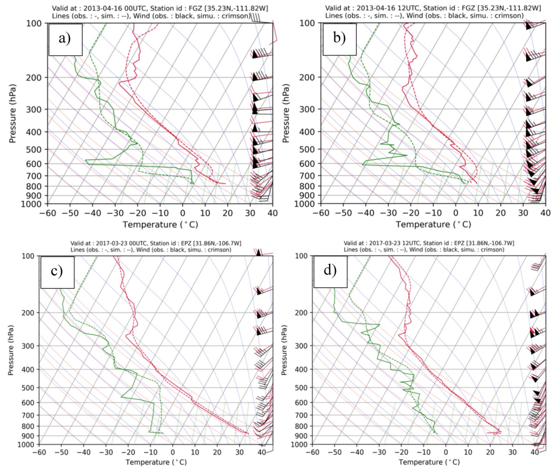
Figure 6. SkewT-LogP diagram at Flagstaff, Arizona (KFGZ) for (a) 0000 UTC and (b) 1200 UTC 16 April 2013, and at Santa Teresa, New Mexico (KEPZ) valid for (c) 0000 UTC and (d) 1200 UTC 23 March 2017.
