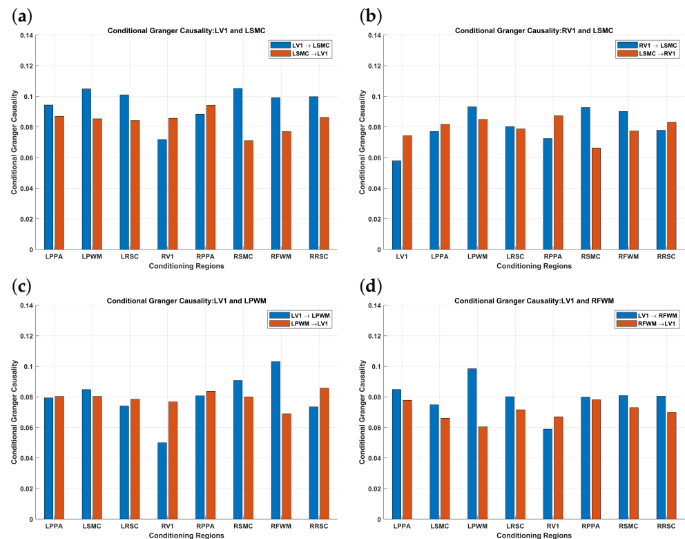
Figure 10. FMRI-based causality analysis using multivariate conditional GC with respect to individual regions. (a) LV1 \rightarrow LSMC , (b) RV1 \rightarrow LSMC , (c) LV1 \rightarrow LPWM , (d) LV1 \rightarrow RFWM . It can be seen that the results of multivariate cCCM and GC are largely consistent for (a,d). However, for (b,c), multivariate cCCM and GC deliver very different results. In particular, for the conditional causality from RV1 \rightarrow LSMC and LV1 \rightarrow LPWM , the results of multivariate cCCM with respect to other individual regions are consistent with their bivariate counterparts and also reflect the impact of inter-region dependence on the conditional causality. However, the corresponding results of multivariate GC with respect to other individual regions vary significantly with the region under consideration, and 50% or more are no longer consistent with those of the bivariate GC.
