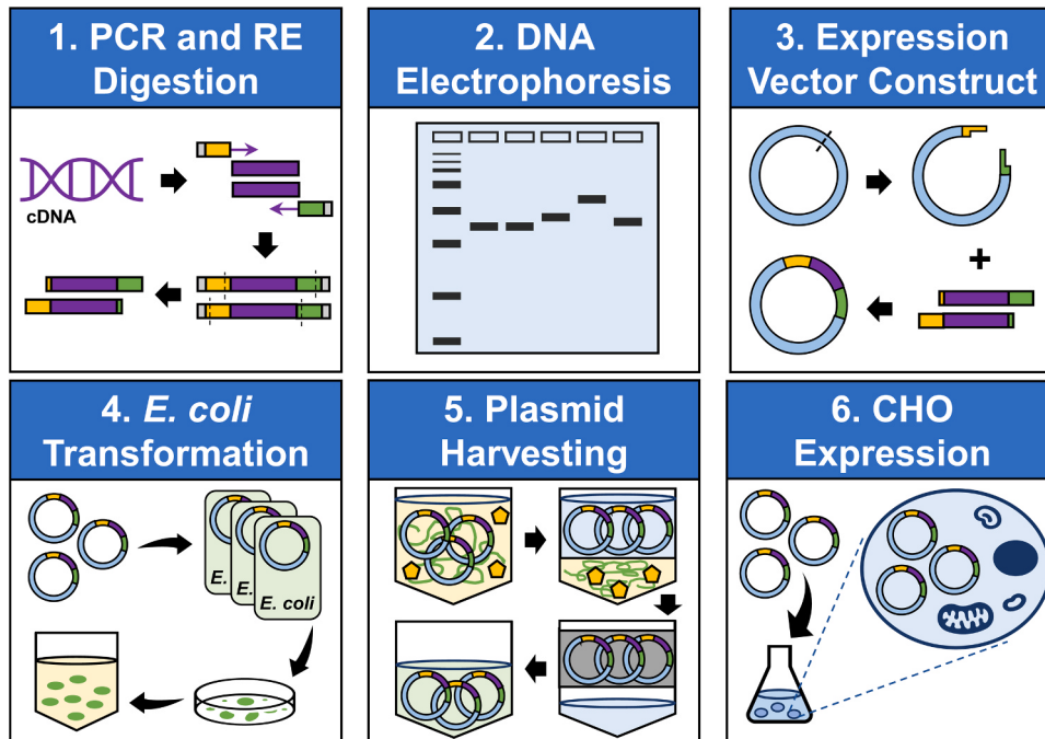
Fig. 1. Genetic engineering pipeline as employed in this study for subclone development and gene functionality analysis. In this study, cellular mRNA was isolated and purified to generate an RNA template of which CHO-K1 cDNA was reversely synthesized. DNA amplification was conducted by PCR to clone target GOI using a pair of forward and reverse primers strategically designed to ensure DNA amplicons containing in-frame expression of GOI and bearing appropriate restriction enzyme sites at both 5' and 3' ends. PCR products were collected and validated via agarose gel electrophoresis, from which DNA fragments containing GOI were extracted and purified. Circular plasmid backbone with different antibiotic resistance genes for individual selection of expression plasmid is digested with restriction enzyme to obtain linearized plasmid construct. For construction of recombinant plasmid DNA, DNA fragments of both GOI and linearized expression vector were ligated with DNA ligase. Host E. coli was then transformed with recombinant plasmid vector construct. Host transformants are selected via the integrated ampicillin marker, after which transformants are recovered and further propagated to obtain plasmid in the concentration of approximately 40 \mu\text{g}/\mu\text{L} per GOI.
