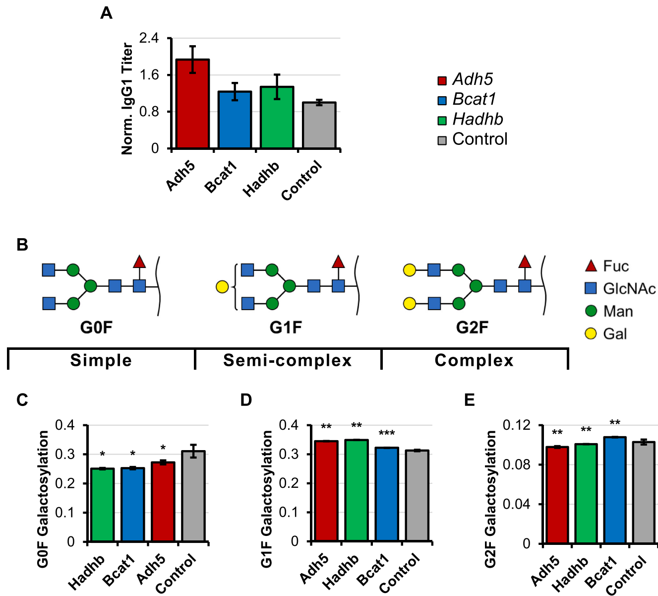
Fig. 6. IgG1 titer and glycosylation profile of genetically engineered CHO cells. (A) Normalized titer profile obtained from each condition against the control. (B) Representative scheme of different glycan structures including a-galactosylated (G0F), mono-galactosylated (G1F), and bi-galactosylated (G2F) biantennary being investigated in the study. Comparison of different glycoform profiles including (C) G0F, (D) G1F, and (E) G2F glycans obtained from purified IgG1 secreted by transfected cells against the control. In this study, batch process of CHO cells was conducted at 0.7 \times 10^6 cells/mL seeding density in 30 mL culture volume. The study was divided into three unique subclone groups. Each subclone was overexpressed with an individual gene of interest via transient transfection at plasmid concentration of 40 \mu\text{g}/\mu\text{L} to cells. A negative control was included in the study (no plasmid transfection occurred). Cells were cultured until cell viability dropped below 80%. Cells for both the control and transfected conditions were derived from the same culture to eliminate variation in growth cycle and other culture conditions. Bars, mean \pm s.d.; n = 3 , * p < 0.05 , ** p < 0.01 , *** p < 0.001 . Statistics by two-tailed t-test.
