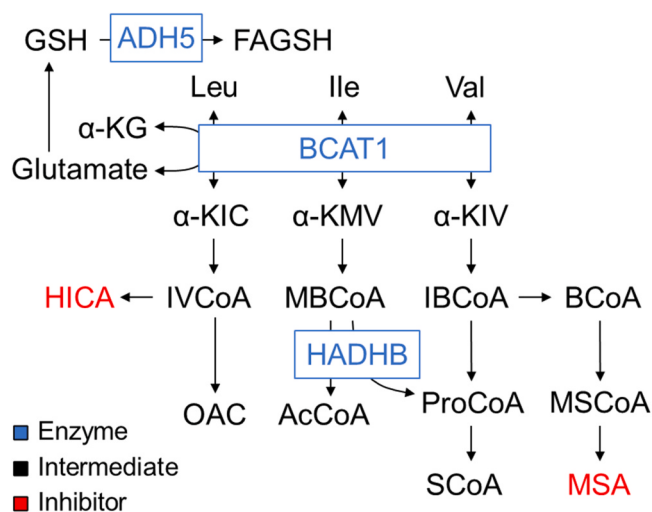
Fig. 3. Genetic engineering strategy targeting accumulation of \alpha -hydroxyisocaproic acid (HICA) and methylsuccinic acid (MSA) accumulation in CHO cells. In this study, metabolic by-products HICA and MSA previously identified to be growth inhibitors accumulated from a batch and fed-batch CHO bioprocess were targeted for genetic engineering study. Genome scale modeling (GEM) revealed additional metabolic pathways that can be controlled through genetic flux modulation. Accumulation of inhibitors can be controlled by up-regulating the expression of characterized genes responsible for modulation of metabolic enzymes that catalyze reaction.
