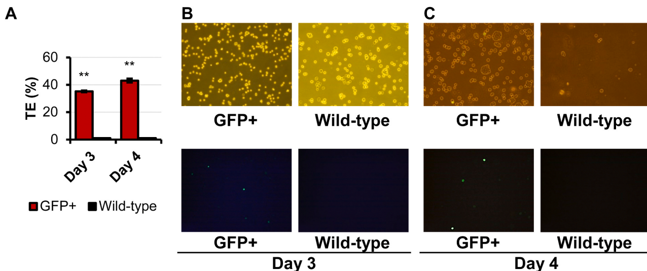
Fig. 4. Validation of recombinant plasmid construct engineered with target gene-of-interest (GOI) and protein expression level. (A) Transfection efficiency (TE) of CHO-S cells as measured through flow cytometric assay on Day 3 and Day 4 post transfection. Imaging of CHO-S cells under normal light and fluorescence light during peak protein production period of cells cultivated in batch process on (B) Day 3 and (C) Day 4. In this study, GFP reporter gene was used as indicator for assessment of translation activity. Cells transfected with GFP-inserted plasmid (GFP+) were compared against wild-type cells (no GFP) to evaluate expression of GFP reporter protein. CHO batch process was conducted at 0.5 \times 10^6 cells/mL seeding density in 30 mL culture volume.
