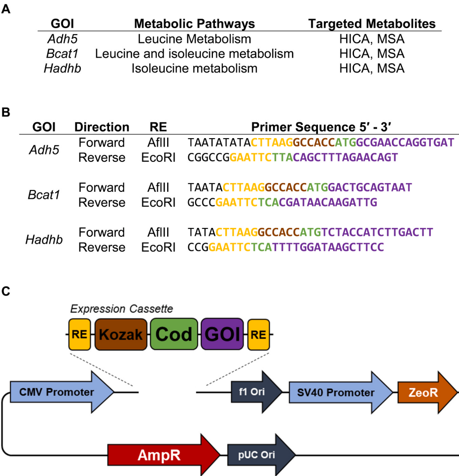
Fig. 2. Cloning of different metabolic gene of interest (GOI) into vector construct assembly. (A) Genes, corresponding metabolic pathways and regulated downstream metabolites (B) Target gene of interest (GOI) flanked by restriction enzymes (RE) along with the corresponding forward and reverse primers as cloned through PCR amplification. (C) Blueprint of vector construct assembly. For (B), to ensure the expression of the GOI, Kozak sequence was engineered into the expression cassette to promote translation activity along with the codons. Different metabolic GOI native to CHO genome were cloned into circular plasmid vector construct for study of their enzymatic activities to control toxic metabolites accumulation when up-regulated in CHO host. Restriction enzyme cutting sites found on the 5' ends of both forward and reverse primers are unique and not present within the sequence of the fragment to be subcloned. Primers are also designed to contain the expressed sequence as the open reading frame to ensure proper in-frame expression. Spacer sequences are introduced at the 5' end of the final primer sequence to ensure proper binding and digestion of the template fragments.
