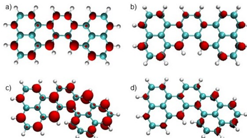
Figure 11. Total MR-AQCC unpaired density plots for a) 16 and c) 19 , respectively, and the corresponding FT-DFT FOD (TPSS-D3 density functional, literature-recommended temperature, 5000 K) for b) 16 and d) 19 . The isovalue = 0.004 e/\text{bohr}^3
