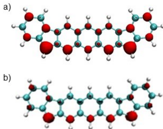
Figure 10. Plots for 12 , cis -diindenoanthracene of the a) MR-AQCC unpaired density and b) FT-DFT FOD (TPSS-D3 density functional, literature-recommended temperature, 5000 K). The isovalue = 0.004 e/bohr 3 .
