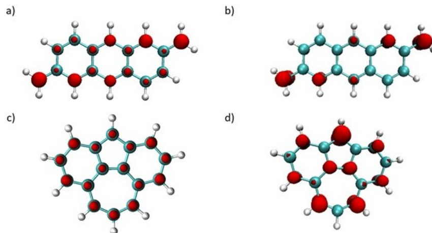
Figure 12. Total MR-AQCC unpaired density plots for a) 28 and c) 29 and the corresponding FT-DFT FOD (TPSS-D3 density functional, literature-recommended temperature, 5000 K) for b) 28 and d) 29 . The isovalue = 0.004 e/bohr 3 .
