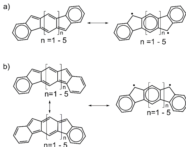
Figure 2. Structures of a) trans -diindenoacenes ( 5-9 ) and b) cis -diindenoacenes ( 10-14 ) showing quinoid Kekulé (left) and biradical (right) resonance structures. The circles indicate Clar's aromatic sextet rings.
