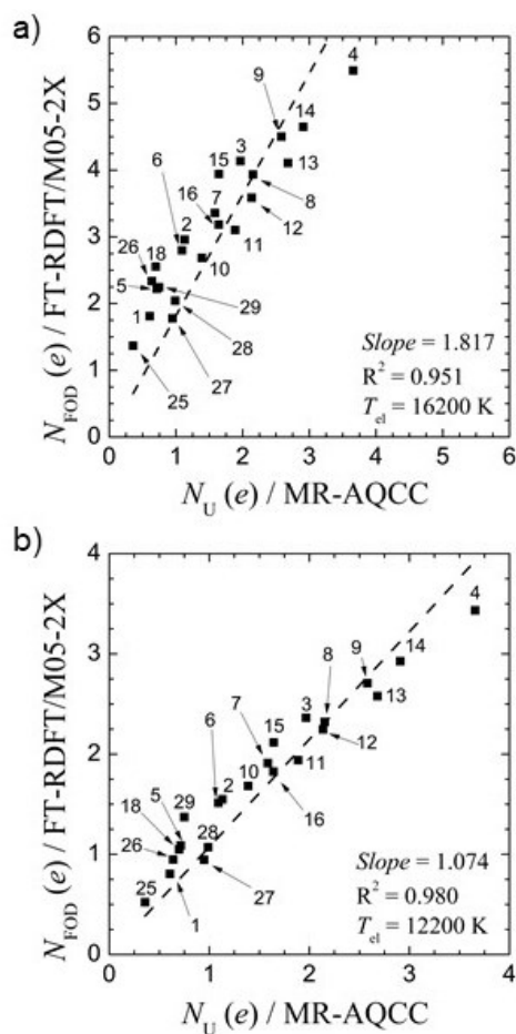
Figure 13: Comparison between MR-AQCC N_U values and FT-RDFT N_{FOD} numbers with the M05-2X density functional for structures with singlet ground electronic state ( 1-16 , 18 , 25-29 ) using the a) literature-recommended FT of 16200 K and b) improved-present FT of 12200 K.
