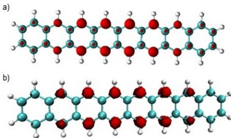
Figure 8. Plots of 8-acene ( 3 ) showing a) for MR-AQCC unpaired density and b) the corresponding FT-DFT FOD (TPSS-D3 density functional, literature-recommended temperature, 5000 K). The isovalue is 0.004 e/bohr 3
