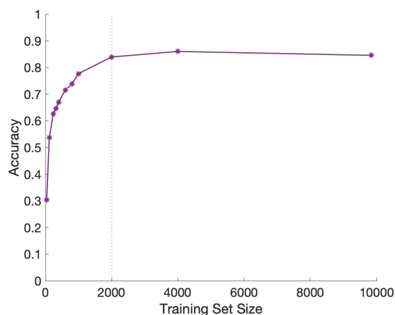
Figure 7. PointNet learning curve: maximum accuracy per training dataset size
