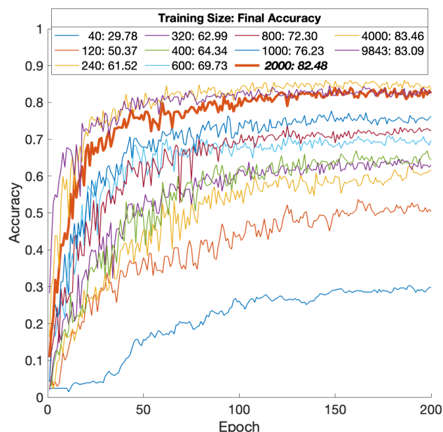
Figure 5. PointNet accuracy versus epoch
