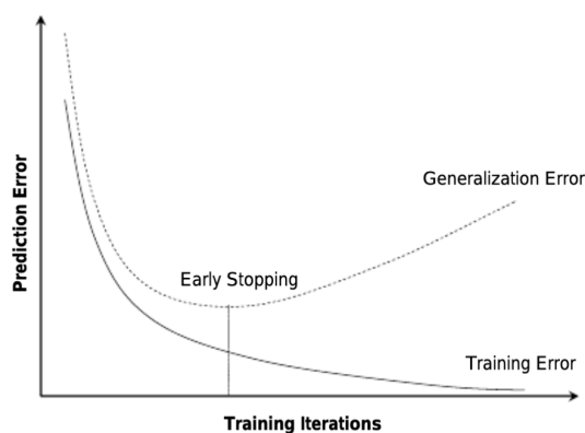
Figure 3. Learning curve showing generalization and training error versus training iterations (Perlich, 2010)
