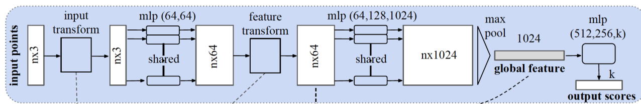
Figure 4. PointNet classification architecture (Qi et al., 2017)
