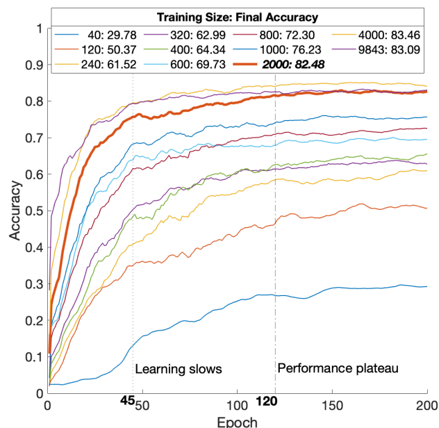
Figure 6. PointNet moving mean accuracy versus epoch
