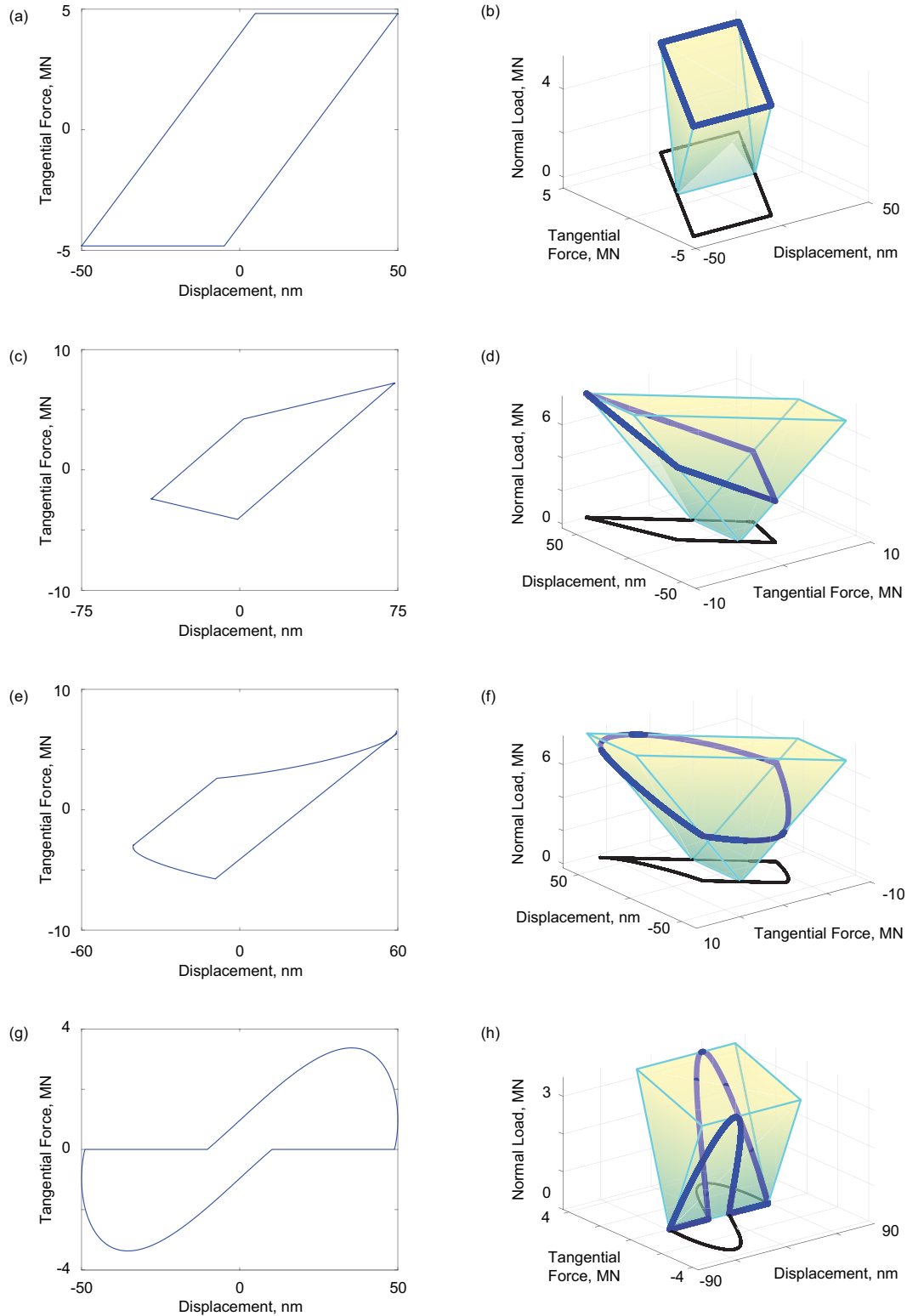
Fig. 6: Hysteresis loops and Masing manifolds for (a)-(b) constant normal force, (c)-(d) sinusoidally varying normal force in phase with the displacement, (e)-(f) sinusoidally varying normal force that is \pi/4 rad out of phase with the displacement, and (g)-(h) sinusoidally varying normal force that goes to zero. All results are from the elastic dry friction model. The black curves on the right plots are the projections of the hysteresis loops onto the N = 0 plane for visualization purposes.
