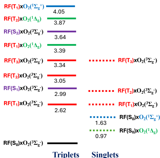
FIG. 6: Energy diagram of the low-lying manifold of singlet and triplet states derived from RF's S 0 , S 1 , S 2 , T 1 , and T 2 and oxygen's 3 Σ g - , 1 Δ g , and 1 Σ g + . Excitation energies in electron-volt relative to the ground state, RF(S 0 ) × O 2 ( 3 Σ g - ).
