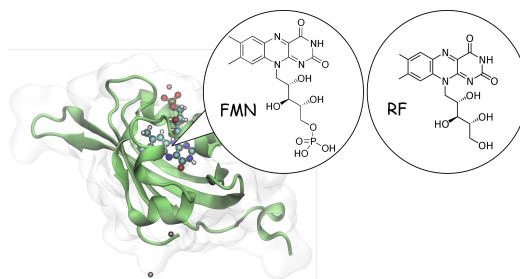
FIG. 1: miniSOG protein. Flavin mononucleotide (FMN) and riboflavin (RF) cofactors are shown in the inserts.
