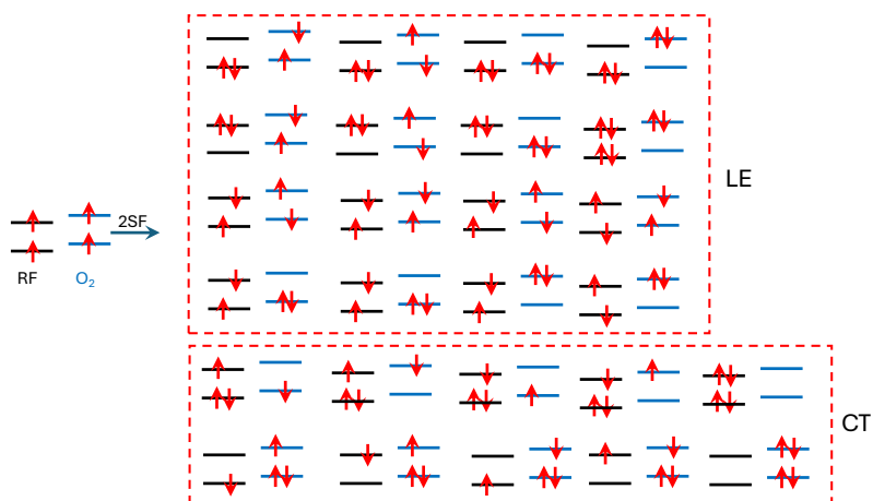
FIG. 3: RAS-2SF reference and target determinants. Singly occupied orbitals are flavin's \pi and \pi^* and oxygen's \pi_x^* and \pi_y^* LE and CT denote local excitations and charge-transfer configurations, respectively.
