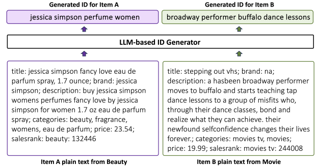
Figure 1: The ID generator takes plain text from each item’s meta textual information and generates abstractive textual IDs for the item’s representation.
