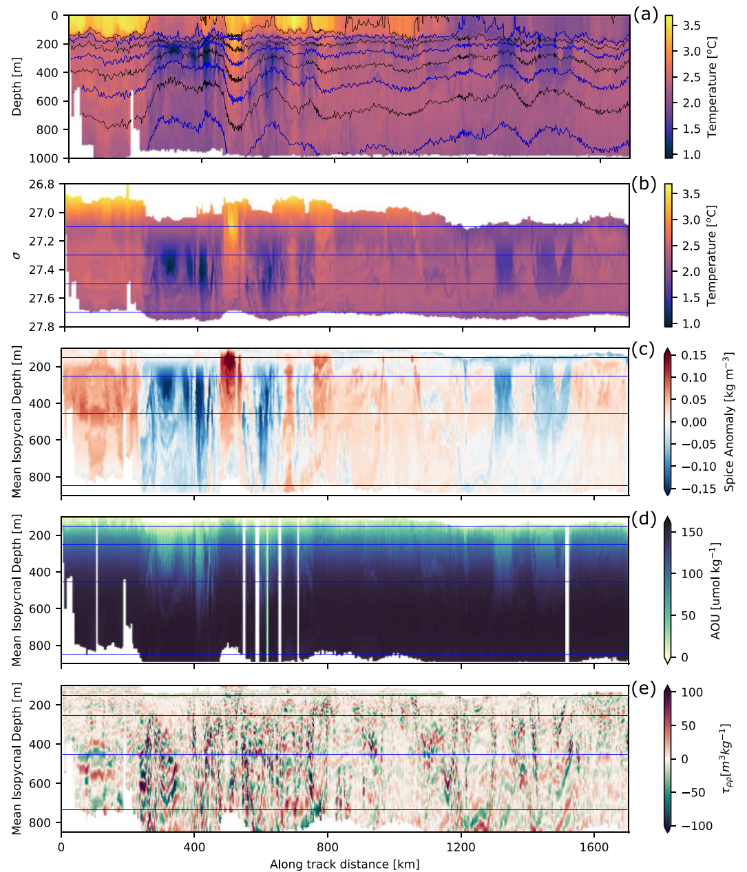
Figure 2. Sections from glider SG660 plotted as a function of along track distance. (a) Conservative temperature and isopycnals (potential density, black and blue contours with levels spaced by 0.1 kg m -3 ) as a function of depth. (b) Conservative temperature as a function of isopycnal potential density. (c) Spice anomaly as a function of mean isopycnal depth. (d) Apparent oxygen utilization (AOU) as a function of mean isopycnal depth. (e) Diapycnal spice curvature, a metric to visually show layering, as a function of mean isopycnal depth. Horizontal blue lines in panels (b–e) indicate the mean depth of the 27.1, 27.3, 27.5, and 27.7 kg m -3 potential density surfaces, which are shown as blue contour lines in (a). Note that the x -axis in these plots is along track distance, which is different from the yearday time shown in Figure 1. A similar plot for SG659 is present in the Supp. Info.
