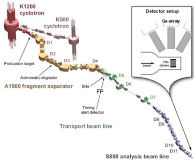
FIG. 1: Sketch of the experimental setup used in the current work. A ^{198}\text{Pt} beam was produced by the NSCL coupled cyclotrons and fragmented on a beryllium target at the start of the A1900 fragment separator. Fragments were transported to the target location of the S800 spectrometer and stopped in a silicon telescope surrounded by GRETINA [23].
