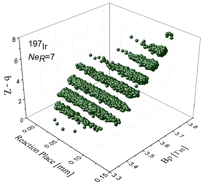
FIG. 4: \text{LISE}^{++} 3D Monte Carlo calculations of the charge state distribution for ^{197}\text{Ir} versus reaction place, assuming post-reaction charge state is Z - q = 7 . The charge state model \text{GLOBAL} was used.
