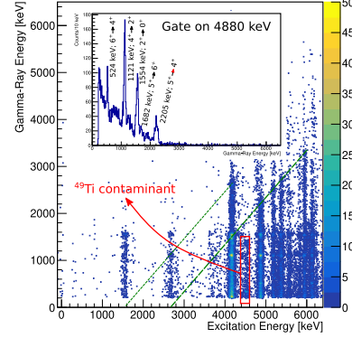
Fig. 5. – Particle- \gamma coincidence matrix measured for the ^{49}\text{Ti}(d, p\gamma)^{50}\text{Ti} reaction with the CeBrA demonstrator and the SE-SPS. The coincident \gamma -ray spectrum when gated on the 4880-keV state of ^{50}\text{Ti} is shown in the inset.
