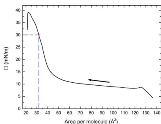
Figure 4. Compression isotherm of the BCM Langmuir film. The arrow indicates the compression direction; the dashed lines point out the deposition parameters.
