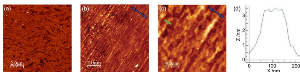
Figure 5. (a) AFM image of a single LB deposition on silicon at \Pi = 12 mN/m, from [33]. (b,c) AFM images of a single LB deposition on silicon at \Pi = 30 mN/m at different magnifications. The blue
