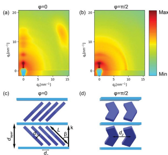
Figure 7. GIWAXS diffraction patterns for different azimuthal orientations of the sample: (a) incidence plane of the X-ray beam parallel to the film compression direction \mathbf{c} ( \varphi = 0 ); (b) incidence plane perpendicular to the film compression direction \mathbf{c} ( \varphi = \pi/2 ). Only the right half of the patterns is shown because of the pattern symmetry. The diffraction intensity is color-coded on a logarithmic scale. On the lower panel, scheme of the layered molecular arrangement for different azimuthal orientations: (c) \varphi = 0 and (d) \varphi = \pi/2 .
