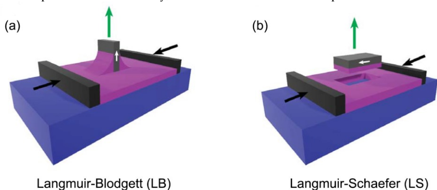
Figure 2. Schematic drawing of the deposition set-up, with the Langmuir film (purple) being transferred from the water (blue) onto the silicon substrate (gray): (a) LB technique used to transfer the first layer; (b) LS technique used to deposit the subsequent 28 layers. The orientation of the substrate during the LB and LS deposition phases is indicated by the in-plane vector \mathbf{c} (white arrow).
