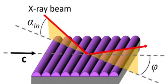
Figure 3. GIWAXS geometry. The drawing highlights the presence of film undulations (purple) along the \mathbf{c} vector, as discussed in section 3.1 and 3.3.
