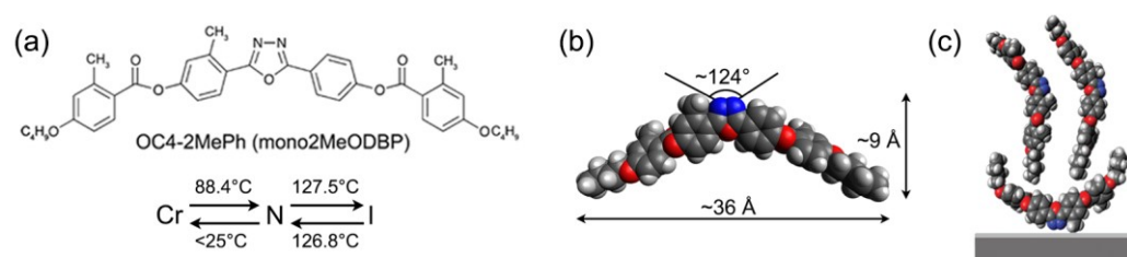
Figure 1. (a) Chemical structure of mesogen OC4-2MePh(mono2MeODBP) with the relative phase transition temperatures on heating and cooling: crystalline phase (Cr) – nematic phase (N) – isotropic phase (I). (b) Optimized molecular geometry. (c) Structure of a Langmuir film deposited on a silicon substrate (with a thin silicon oxide layer at the interface), according to [33].
