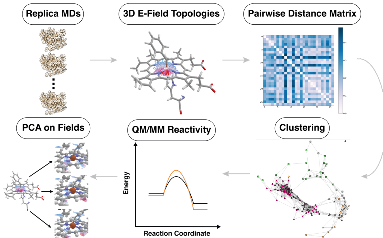
Figure 2. This study's approach measures electrostatic preorganization by analyzing the heterogeneous electric field topology across replica MD simulations. It further involves comparing these topologies using a pairwise distance matrix, clustering based on similarity, and then quantifying reactivity through QM/MM methods. The reactivity difference is chemically elucidated using Principal Component Analysis.
