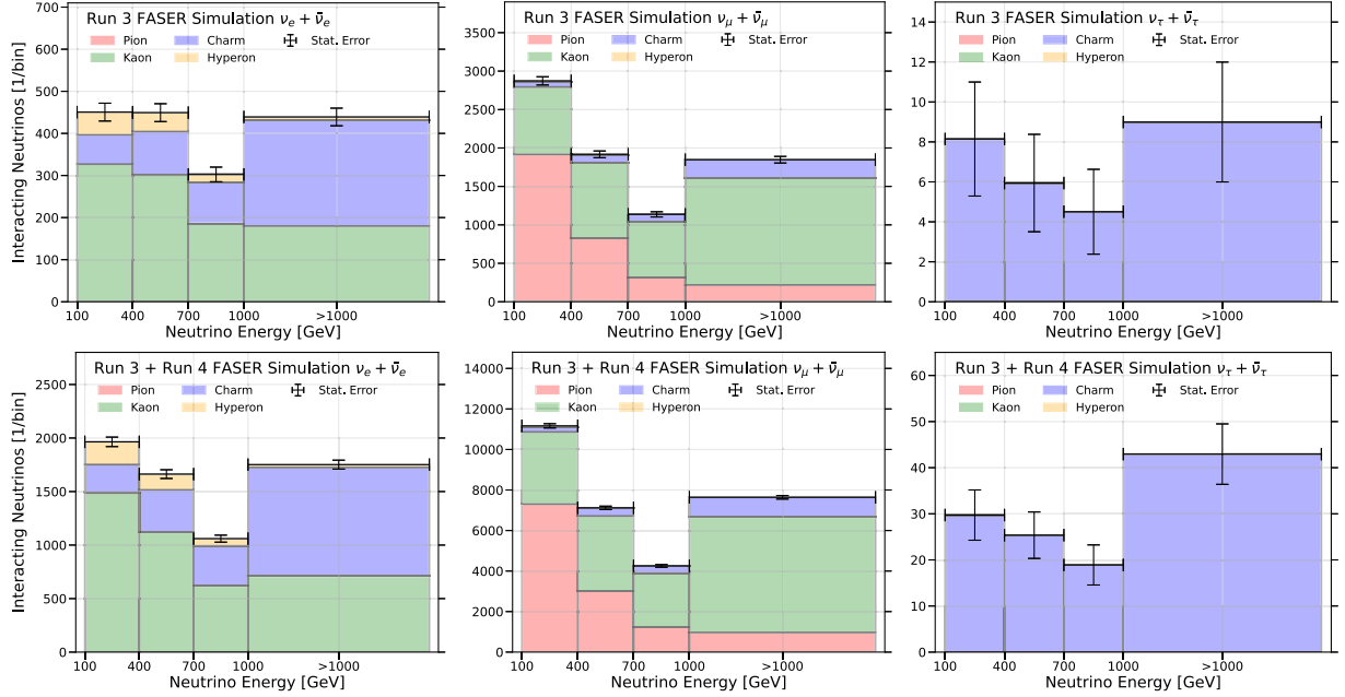
FIG. 8. Binned energy spectra for electron (left), muon (center), and tau (right) neutrinos interacting in \text{FASER}\nu at LHC Run 3 with a total integrated luminosity of 250 \text{ fb}^{-1} (upper panels) and at LHC Run 3 + Run 4 with a total integrated luminosity 930 \text{ fb}^{-1} (lower panels). For each bin, the neutrinos are separated by their parent hadrons: pions (red), kaons (green), charm hadrons (blue), and hyperons (yellow). Hadron production and decay of light (charm) hadrons are modeled by EPOS-LHC (POWHEG+PYTHIA8.3). Also shown are statistical errors per bin, defined as \sqrt{N_{\text{bin}}} , which demonstrate that Run 3 measurements will have sufficient statistics to be sensitive to components of neutrinos from the different parent hadrons.
