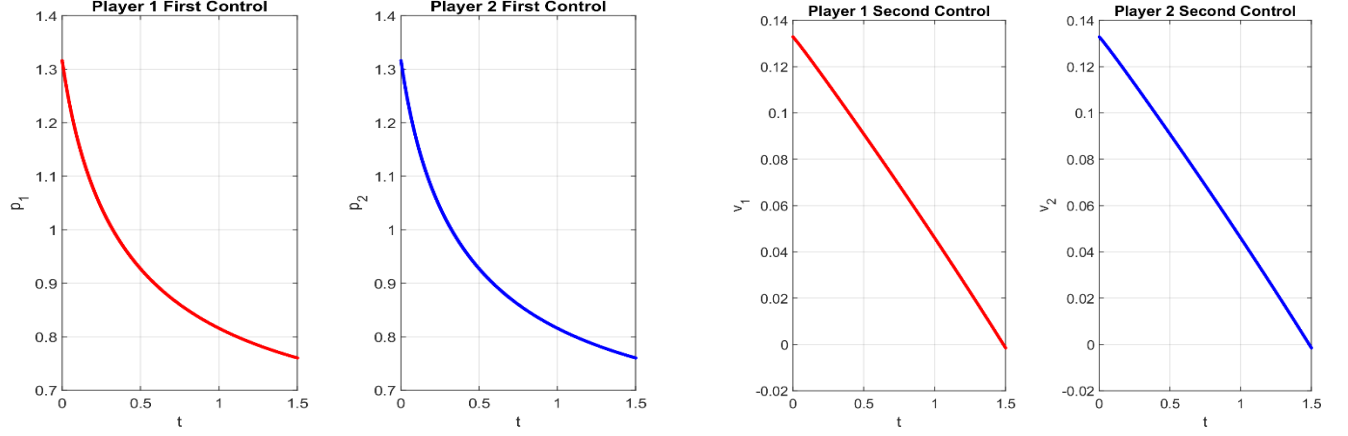
Fig. 3: Trajectories of Player 1 and 2's Optimal Control p_i(t) and v_i(t)
