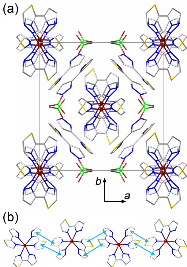
Fig. 3 (a) The crystal packing of 3 \cdot 2(3tpH) viewed down the c axis to reveal columns of [Fe(3tpH)_3]^{2+} cations. The unit cell is indicated with solid gray lines. The H atoms are omitted for clarity. The disorders of the 3tpH ligands and ClO_4^- anions are not shown. (b) A side view of a single column of cations, showing \pi - \pi interactions with light-blue double arrows. Color scheme: Fe = garnet, S = gold, Cl = green, O = red, N = blue, C = gray.
