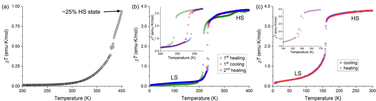
Fig. 4 The temperature dependence of the \chi T product for complexes 1 (a), 2-MeOH (b), and 3 \cdot 2(3tpH) (c), measured under the cooling or heating rate of 2 \text{ K min}^{-1} . The order of processes indicated in the legends corresponds to the actual sequence of measurements performed in the heating and cooling modes. The insets in panels (b) and (c) show an enlarged region of each plot around the spin-transition temperature ( T_{1/2} ). Note that in the case of complex 2 the interstitial solvent has been lost by the end of the first heating cycle (see the discussion in the text for details).
