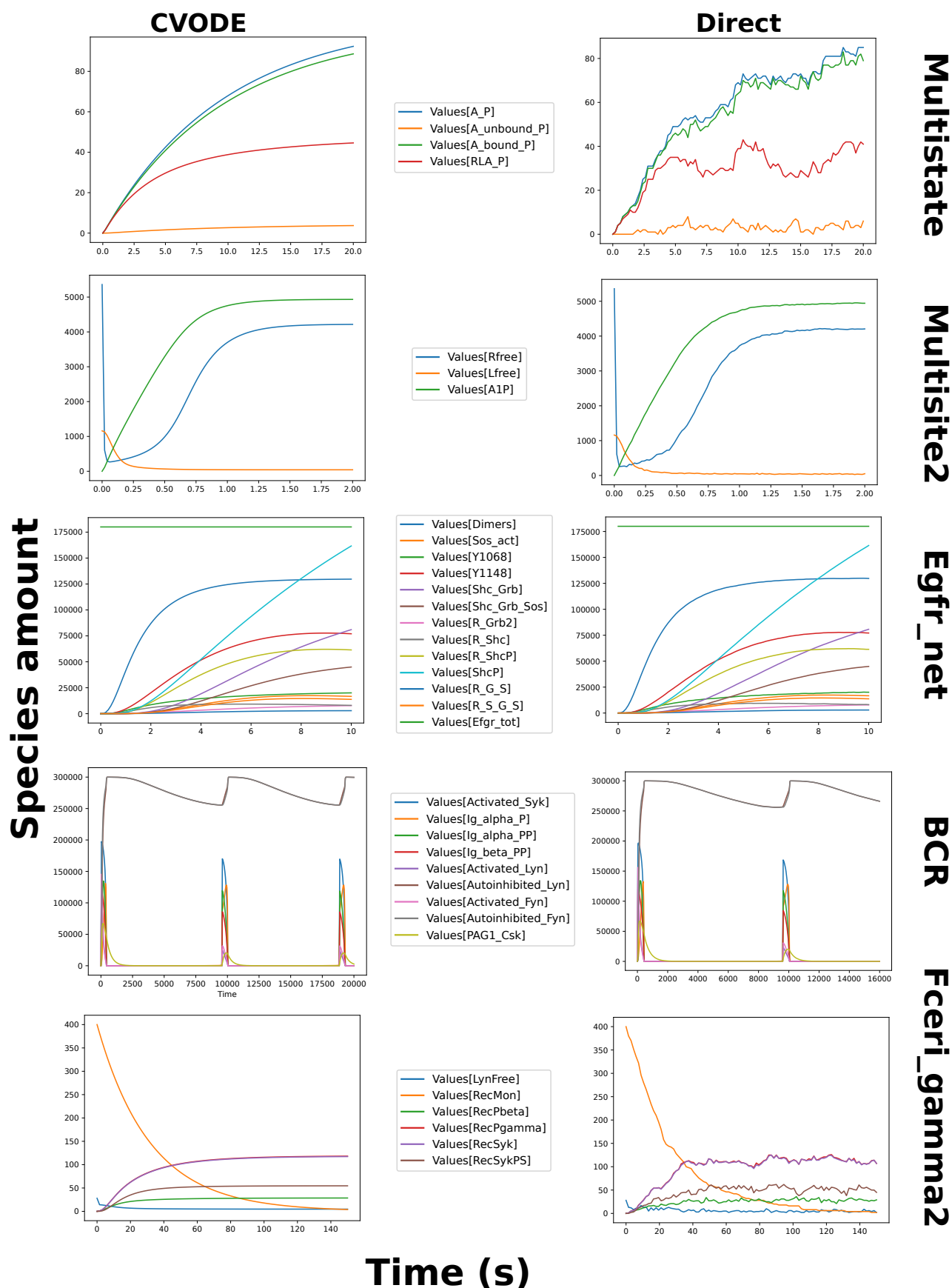
Figure F.8: COPASI benchmark simulation time trajectories. All models are simulated until they reach their (approximate) steady state (same time point which was used for the benchmarks in Fig. 3). The simulation trajectories correspond to those of the other tools, suggesting that the models are correctly interpreted.
