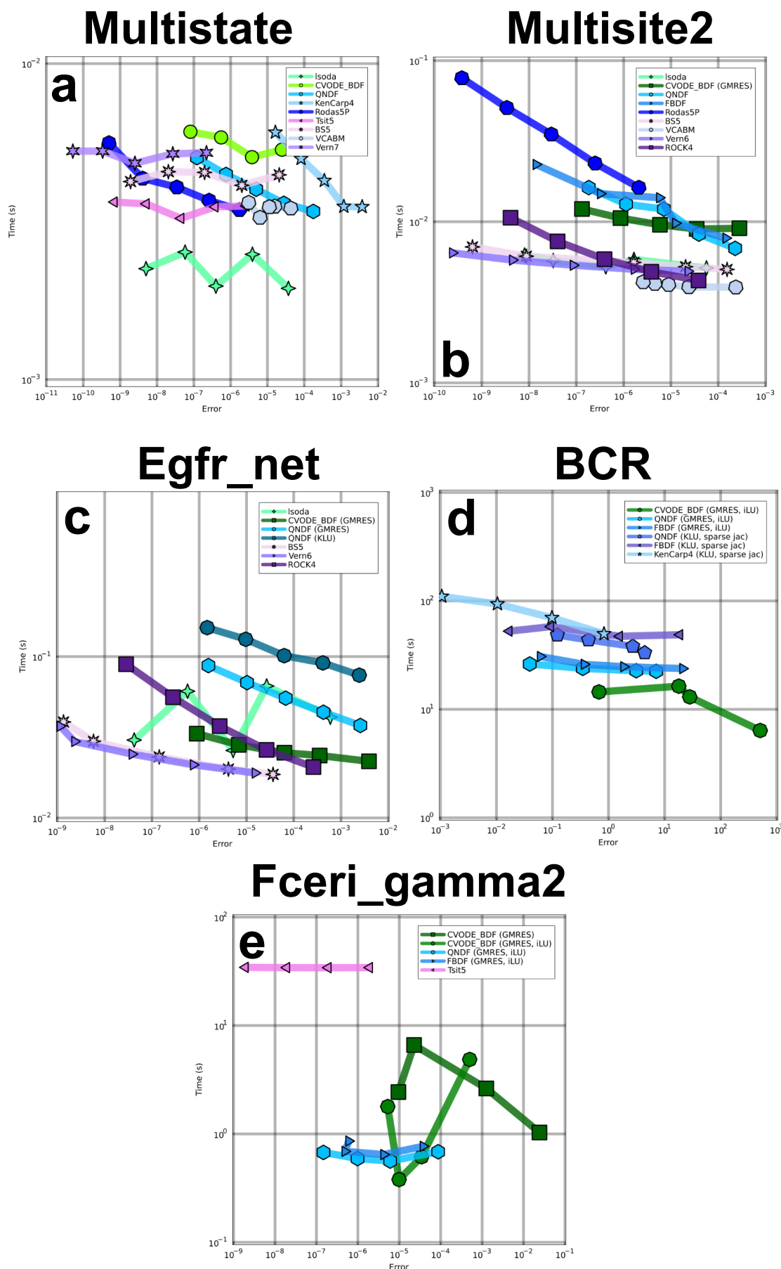
Figure E.1: Work-precision diagrams for selected Julia ODE solvers (and options). Native Julia solvers typically have smaller errors (compared to lsoda and CVODE) when tolerances are kept identical. The simulation options used for this figure are drawn from the list in Supplementary Section B.
