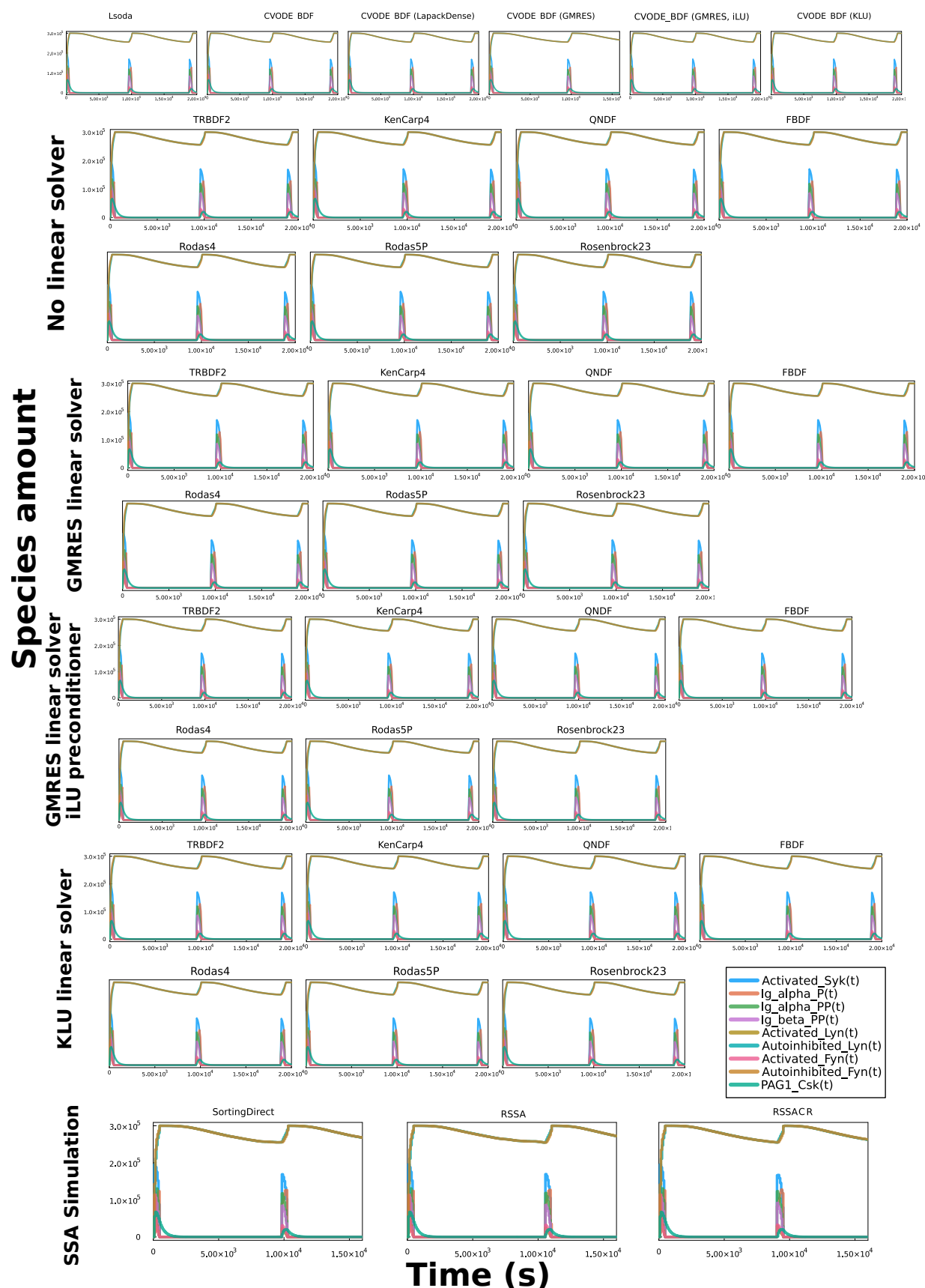
Figure F.4: Catalyst benchmark simulation time trajectories for the BCR model. The BCR model is simulated until it reaches its (approximate) steady state at t = 10,000 seconds (same time point which was used for the benchmarks in Fig. 3). It was simulated using both ODE and SSA methods. The time of the SSA simulation's pulse initiation is variable, and hence the system was resimulated to ensure that a pulse was initiated in the simulation. The simulation trajectories correspond to those of the other tools, suggesting that the models are correctly interpreted.
